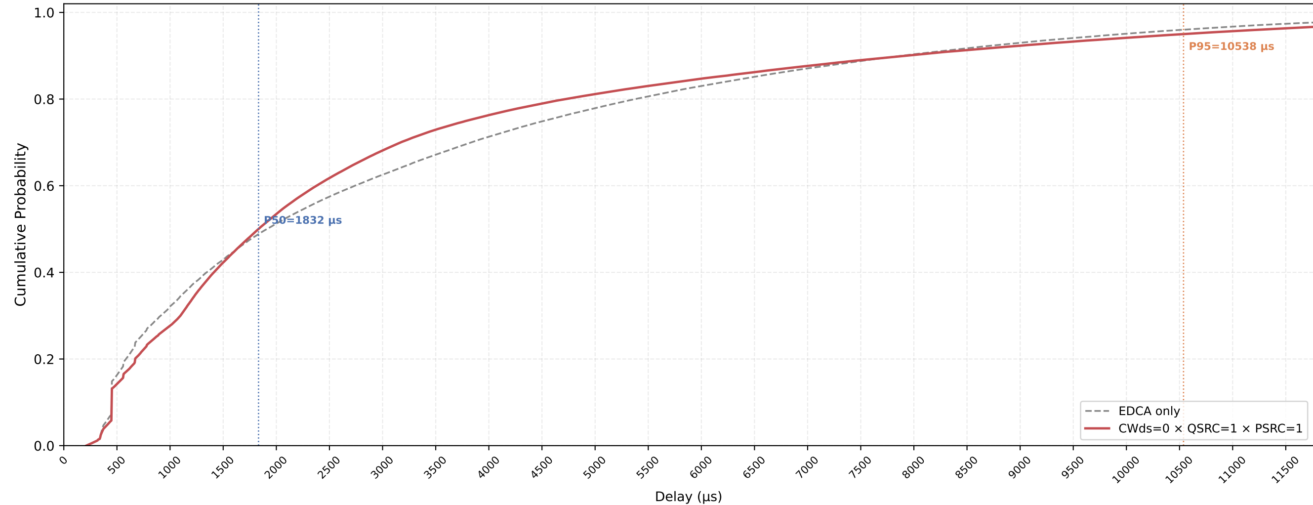
VO (all STAs) Delay CDF — CWds=0 × QSRC=1 × PSRC=1 nSta=30, nPedca=30, 1Mbps, avg of 10 runs
