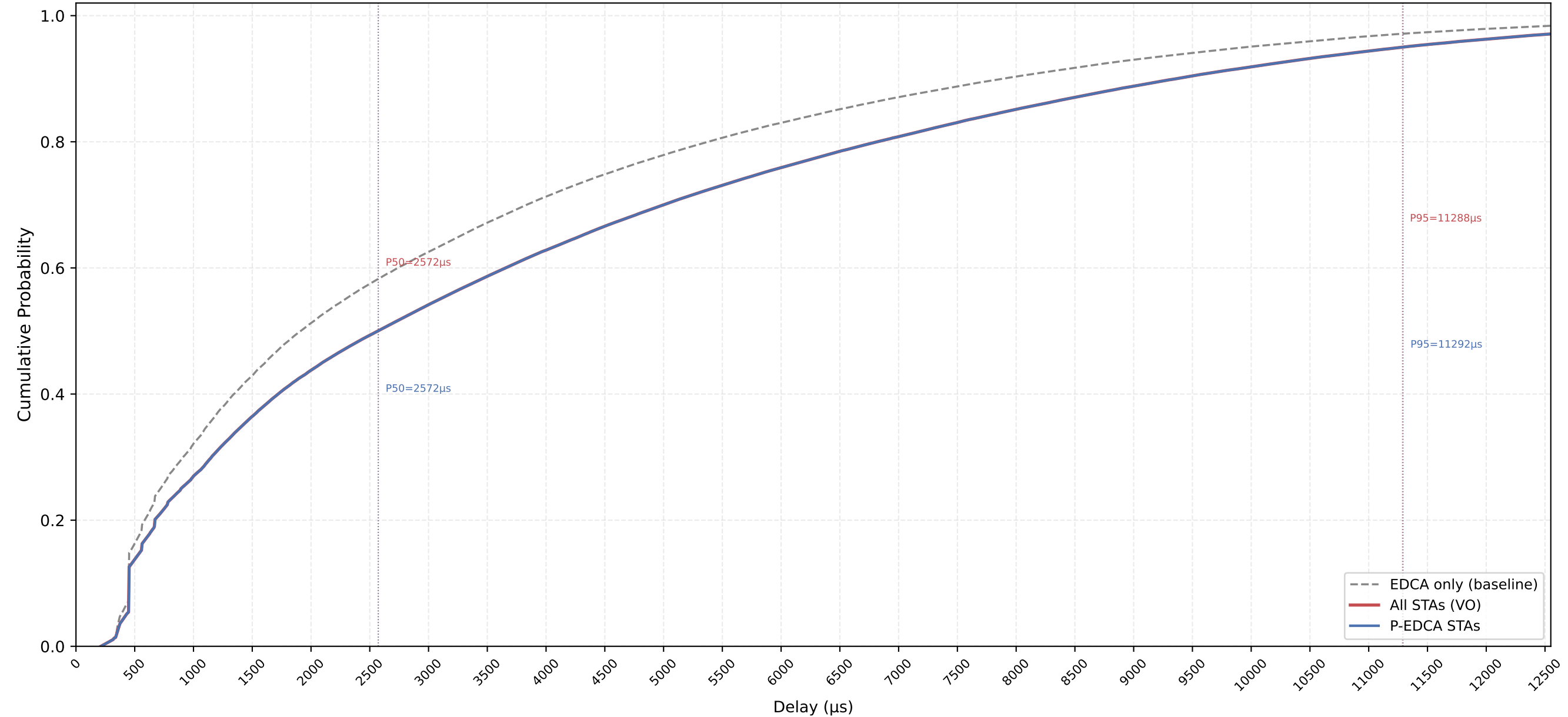
VO Delay CDF — P-EDCA / Legacy / All | CWds=0 × QSRC=5 × PSRC=1 nSta=30, nPedca=30/30, 1Mbps, avg of 10 runs
