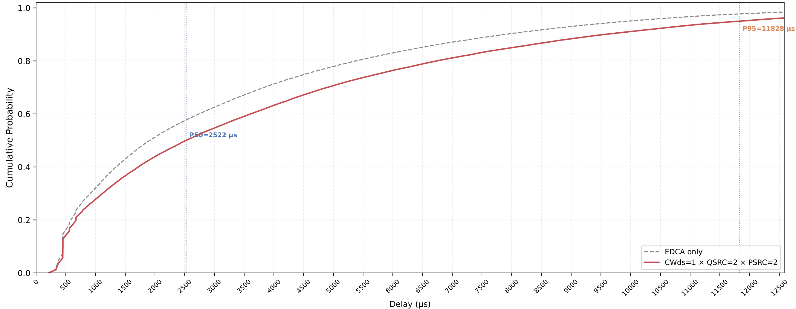
Legacy STA VO Delay CDF — CWds=1 × QSRC=2 × PSRC=2 nSta=30, nPedca=15, 1Mbps, avg of 10 runs
