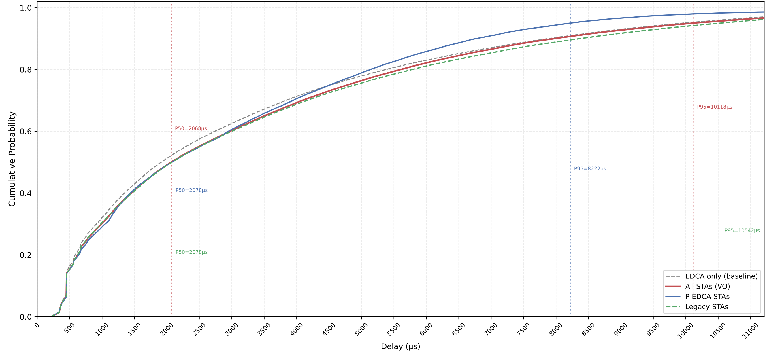
VO Delay CDF — P-EDCA / Legacy / All | CWds=1 × QSRC=3 × PSRC=1 nSta=30, nPedca=5/30, 1Mbps, avg of 10 runs
