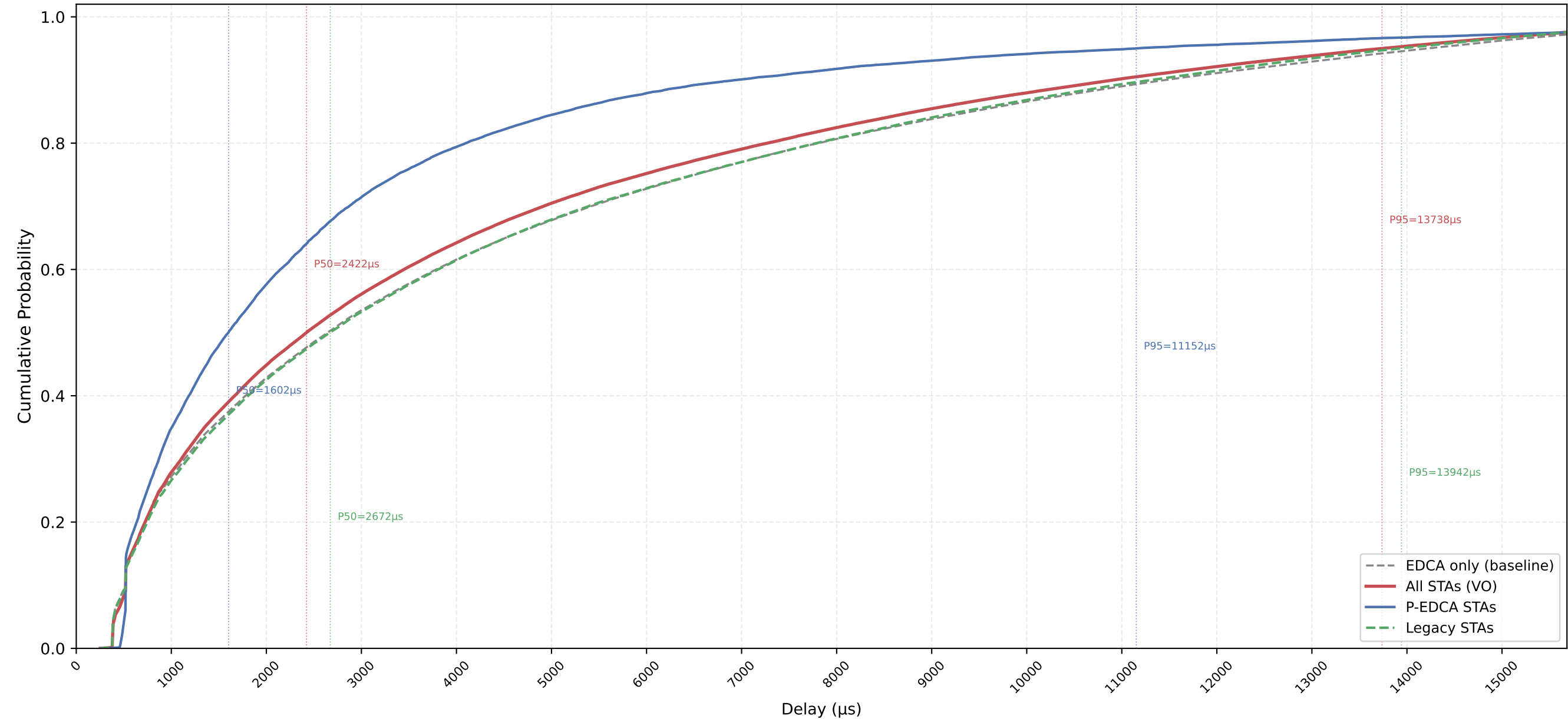
VO Delay CDF — P-EDCA / Legacy / All | CWds=0 × QSRC=0 × PSRC=1 nSta=30, nPedca=5/30, 0.5Mbps, avg of 10 runs
