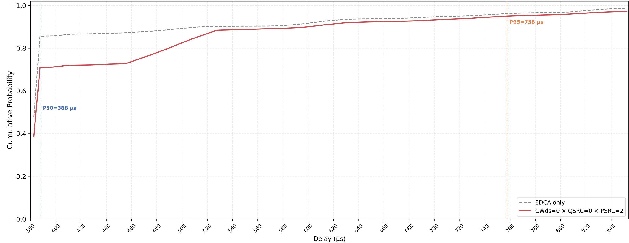
VO (all STAs) Delay CDF — CWds=0 × QSRC=0 × PSRC=2 nSta=30, nPedca=5, 0.1Mbps, avg of 10 runs
