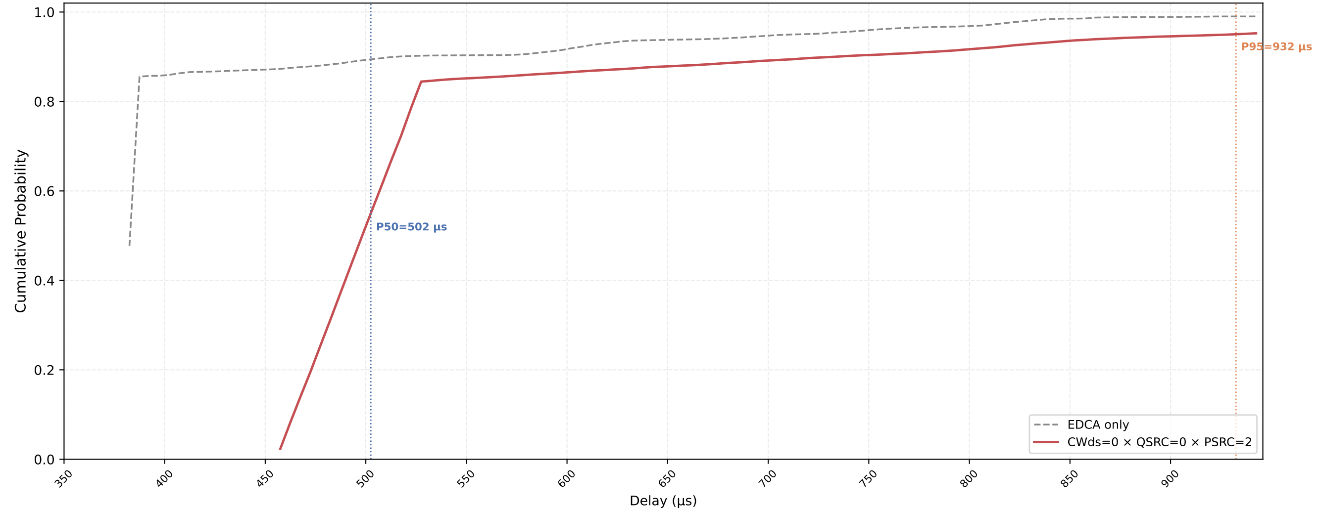
VO (all STAs) Delay CDF — CWds=0 × QSRC=0 × PSRC=2 nSta=30, nPedca=30, 0.1Mbps, avg of 10 runs
