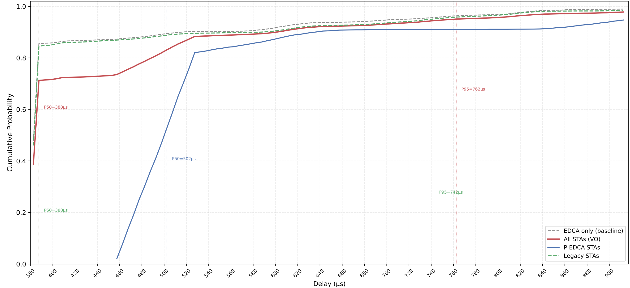
VO Delay CDF — P-EDCA / Legacy / All | CWds=0 × QSRC=0 × PSRC=3 nSta=30, nPedca=5/30, 0.1Mbps, avg of 10 runs
