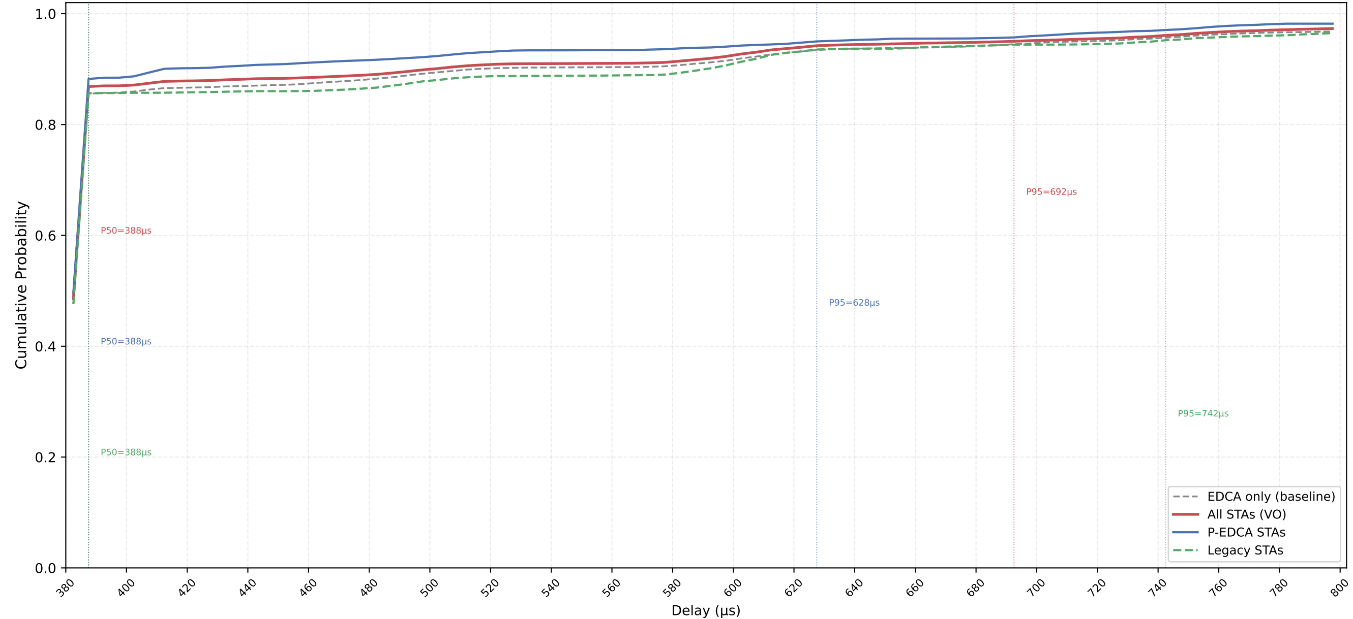
VO Delay CDF — P-EDCA / Legacy / All | CWds=0 × QSRC=1 × PSRC=1 nSta=30, nPedca=15/30, 0.1Mbps, avg of 10 runs
