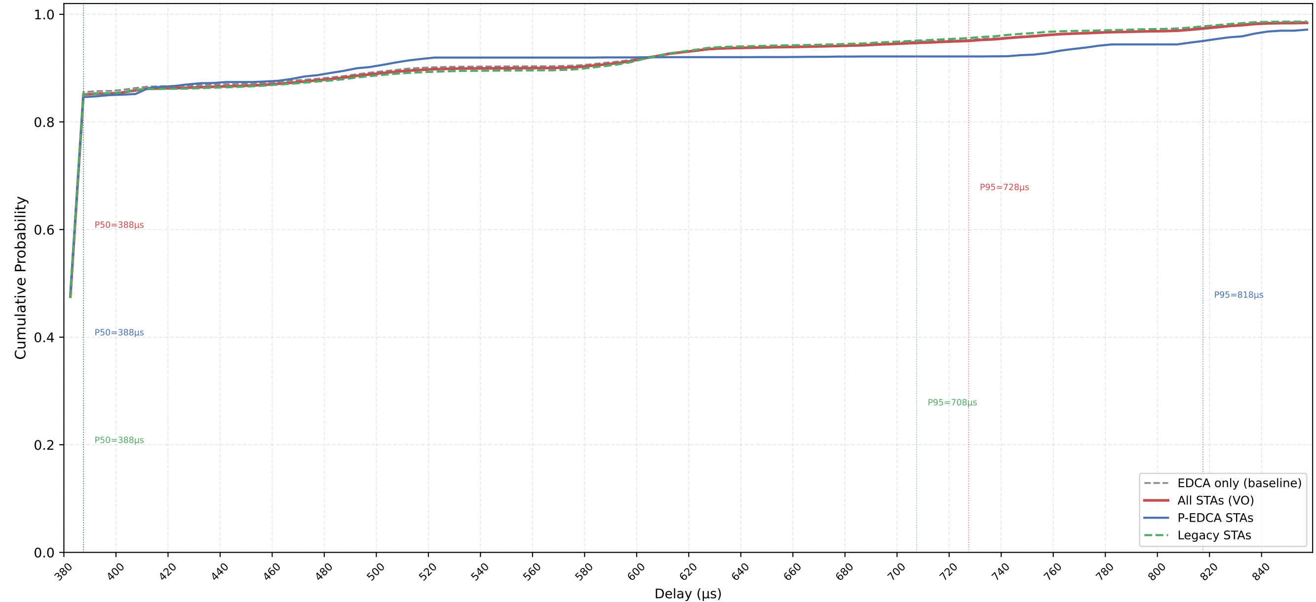
VO Delay CDF — P-EDCA / Legacy / All | CWds=0 × QSRC=1 × PSRC=2 nSta=30, nPedca=5/30, 0.1Mbps, avg of 10 runs
