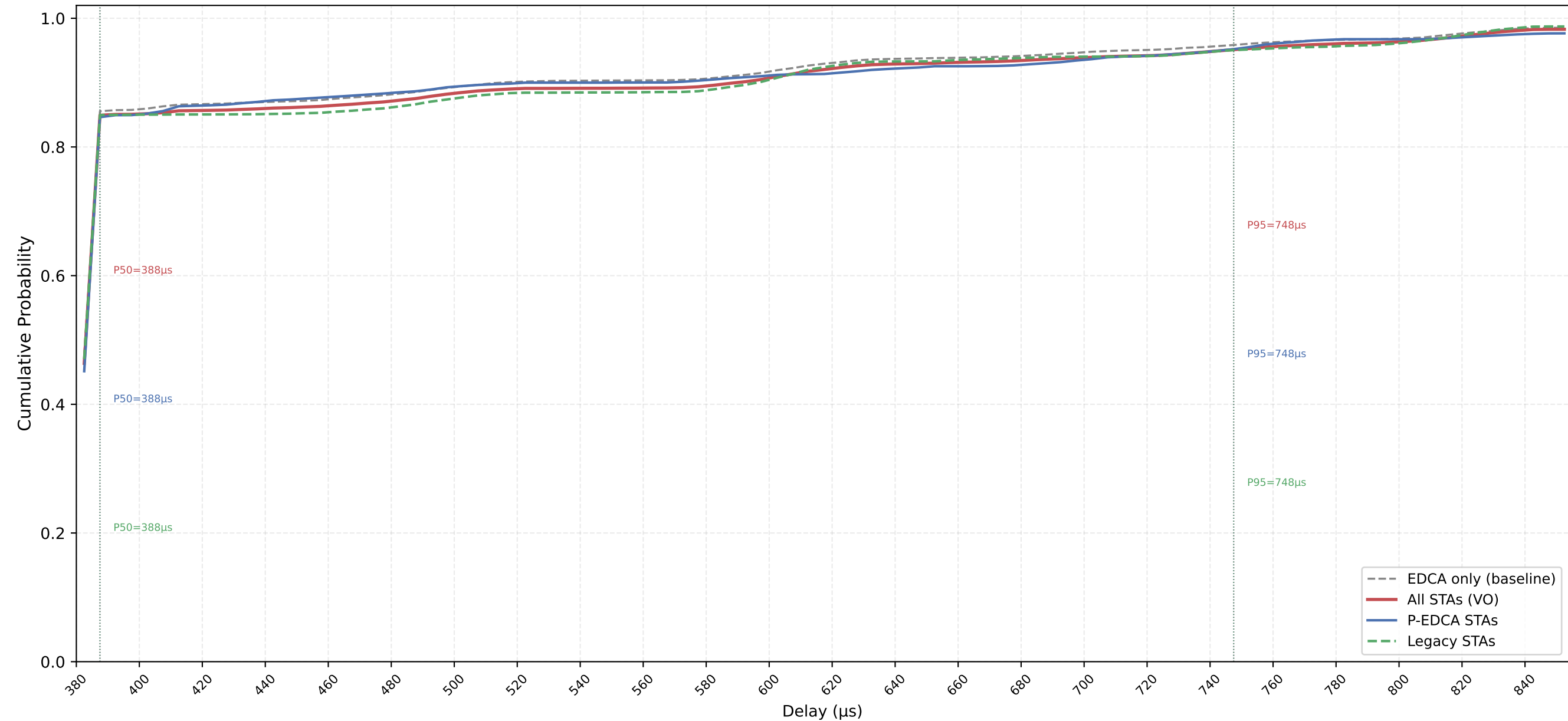
VO Delay CDF — P-EDCA / Legacy / All | CWds=0 × QSRC=1 × PSRC=3 nSta=30, nPedca=15/30, 0.1Mbps, avg of 10 runs
