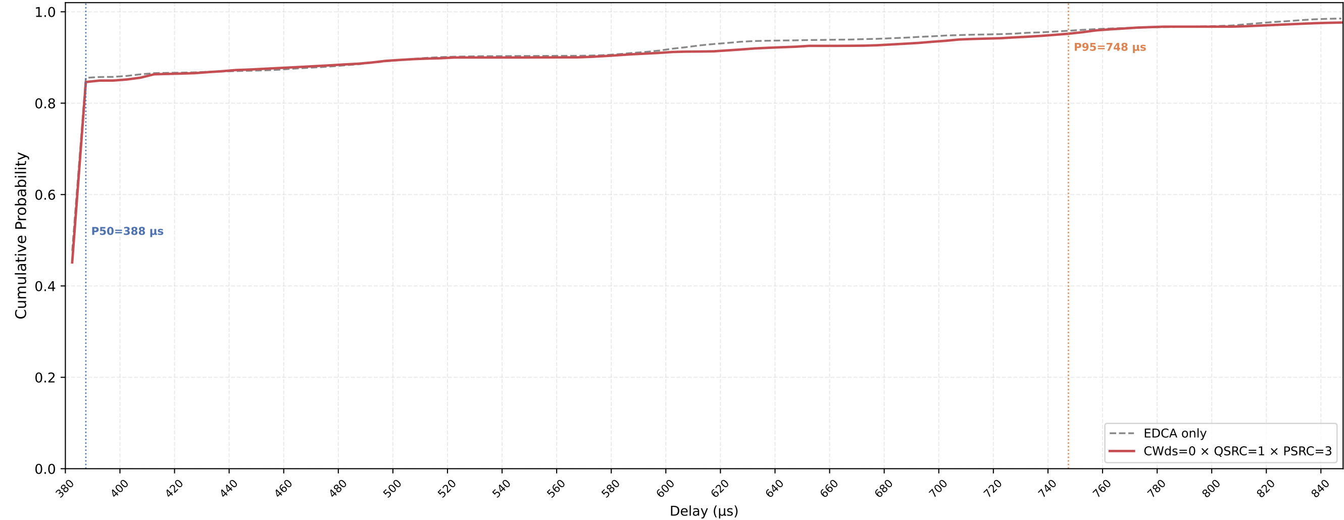
P-EDCA STA VO Delay CDF — CWds=0 × QSRC=1 × PSRC=3 nSta=30, nPedca=15, 0.1Mbps, avg of 10 runs
