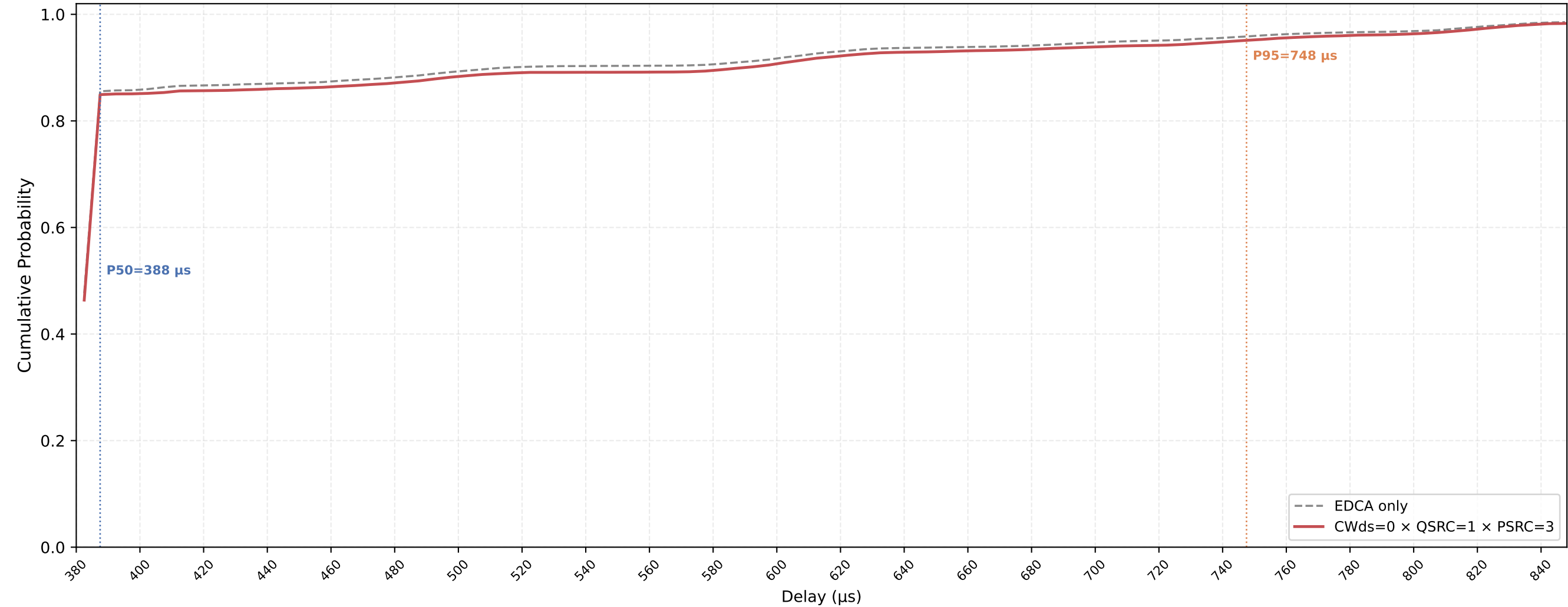
VO (all STAs) Delay CDF — CWds=0 × QSRC=1 × PSRC=3 nSta=30, nPedca=15, 0.1Mbps, avg of 10 runs
