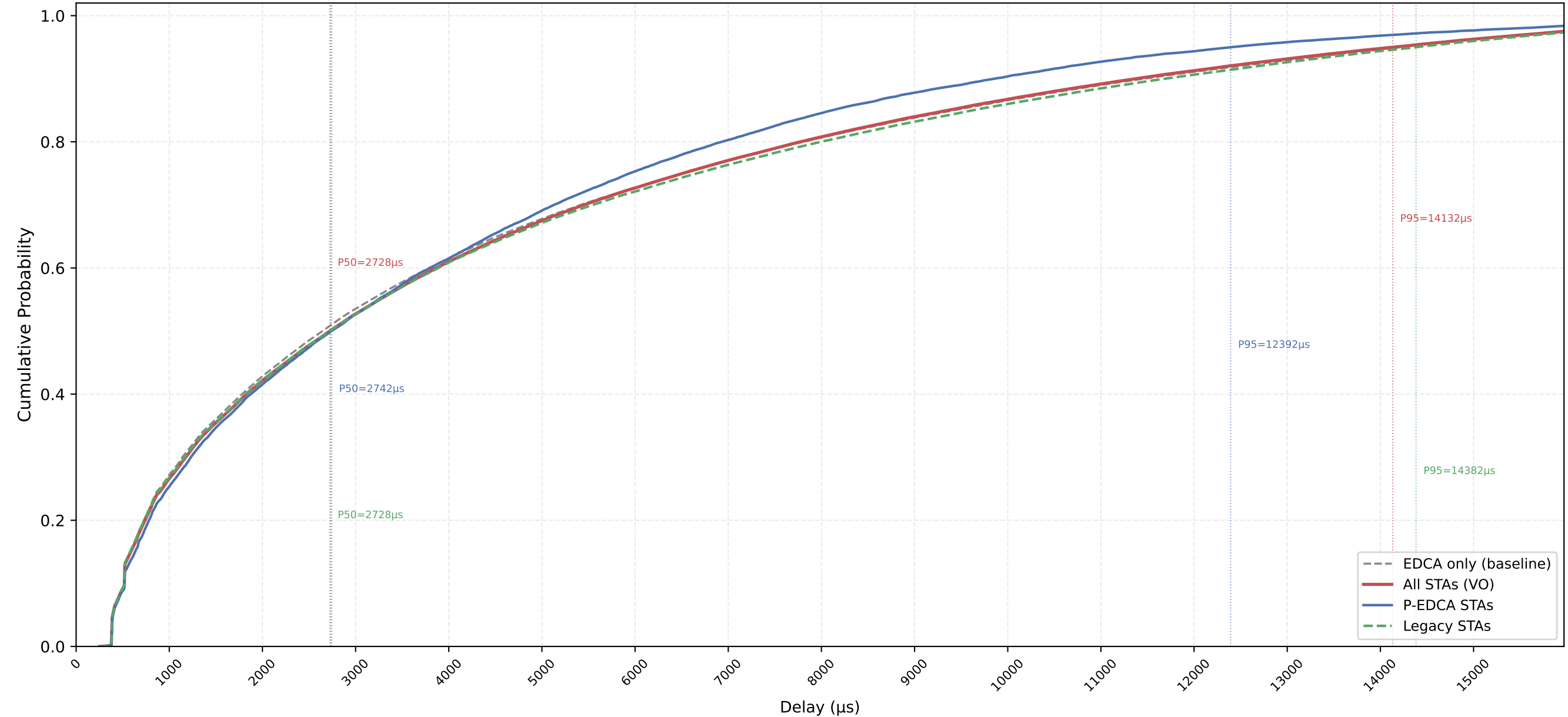
VO Delay CDF — P-EDCA / Legacy / All | CWds=0 × QSRC=2 × PSRC=1 nSta=30, nPedca=5/30, 0.5Mbps, avg of 10 runs
