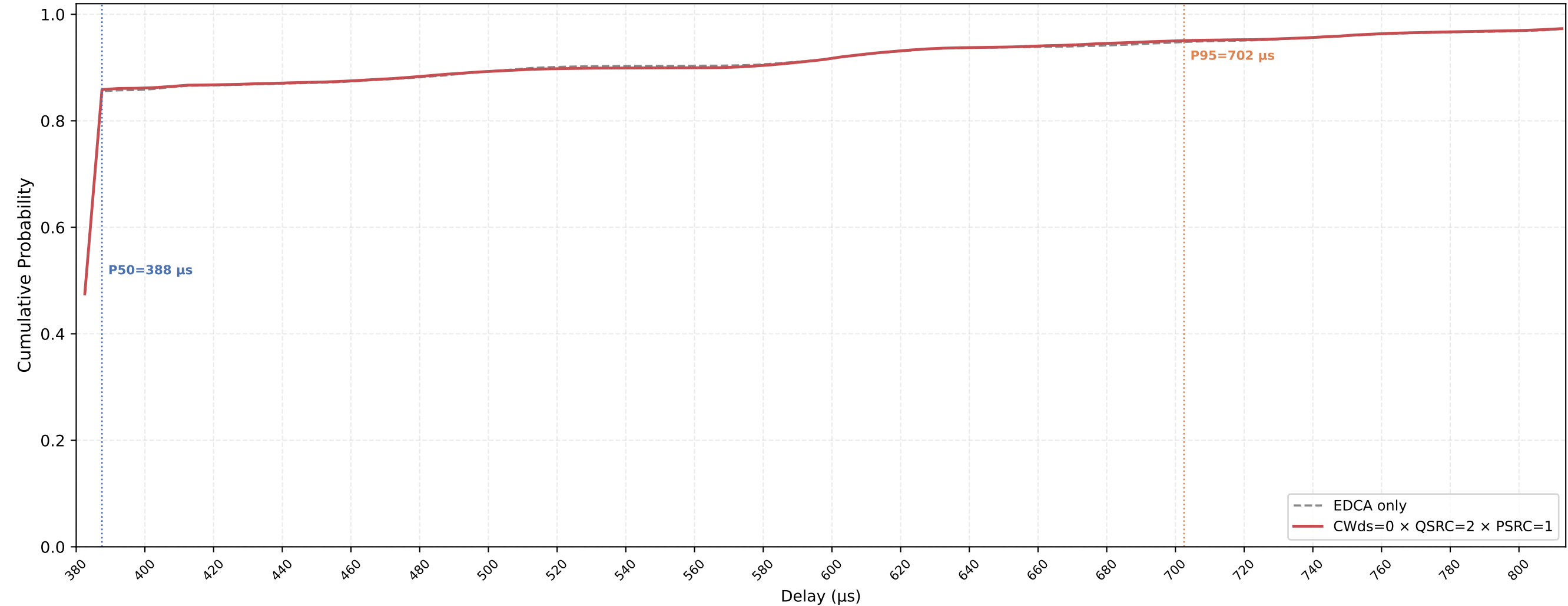
P-EDCA STA VO Delay CDF — CWds=0 × QSRC=2 × PSRC=1 nSta=30, nPedca=30, 0.1Mbps, avg of 10 runs
