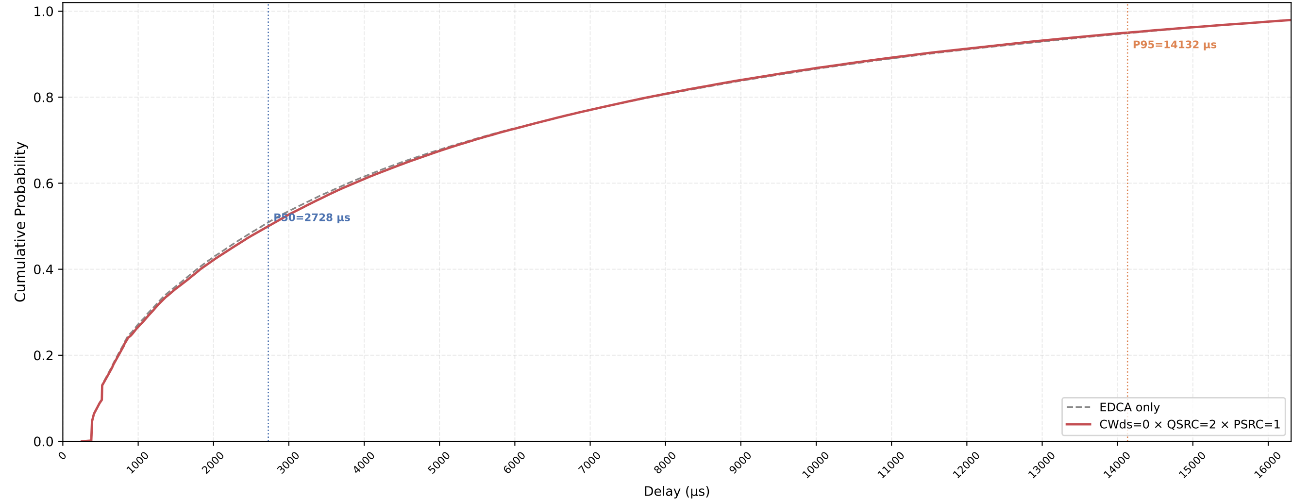
VO (all STAs) Delay CDF — CWds=0 × QSRC=2 × PSRC=1 nSta=30, nPedca=5, 0.5Mbps, avg of 10 runs
