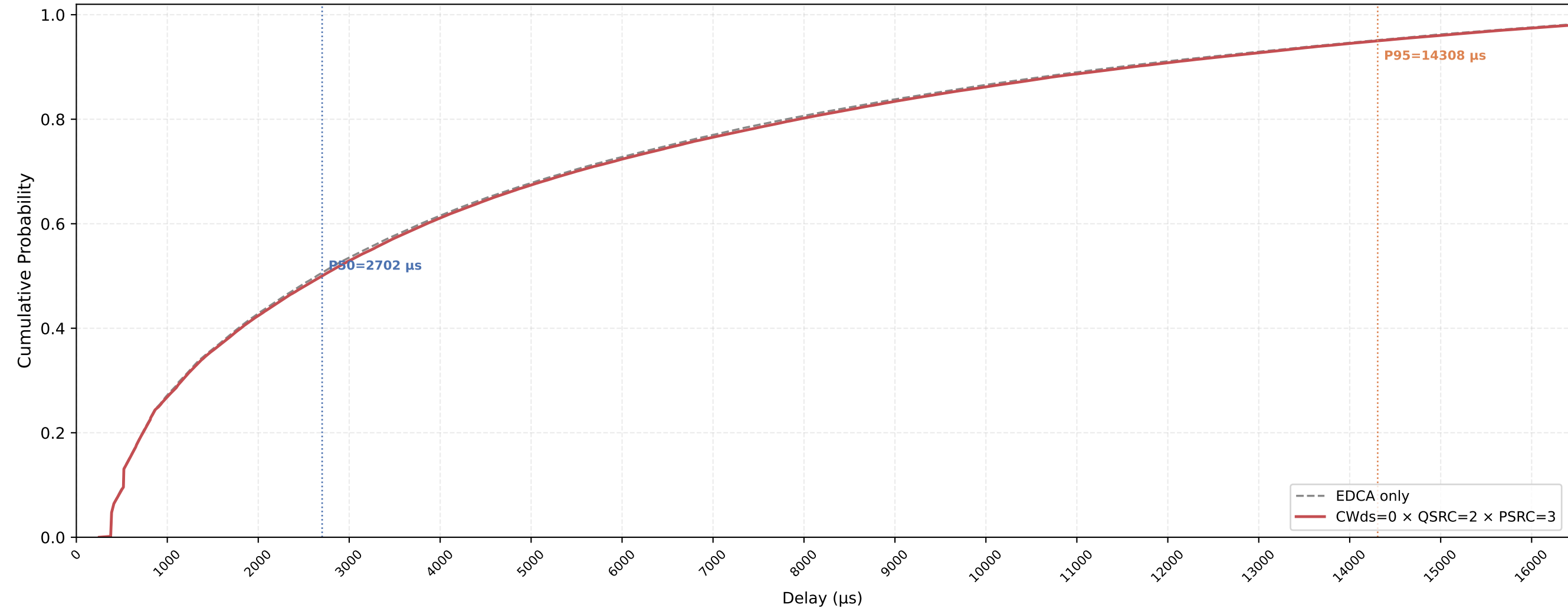
Legacy STA VO Delay CDF — CWds=0 × QSRC=2 × PSRC=3 nSta=30, nPedca=5, 0.5Mbps, avg of 10 runs
