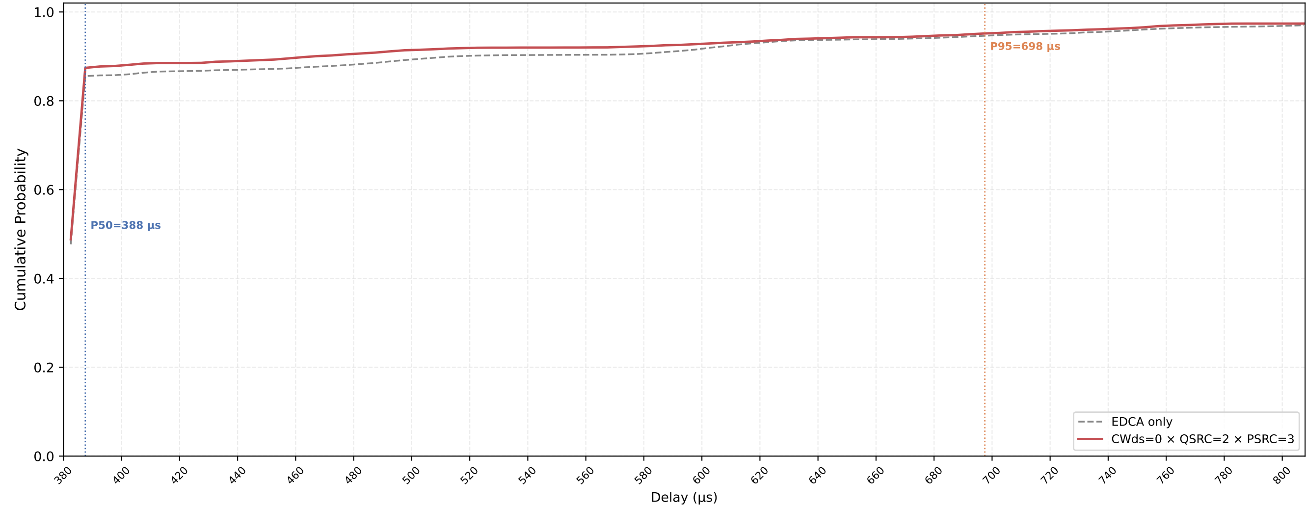
P-EDCA STA VO Delay CDF — CWds=0 × QSRC=2 × PSRC=3 nSta=30, nPedca=15, 0.1Mbps, avg of 10 runs
