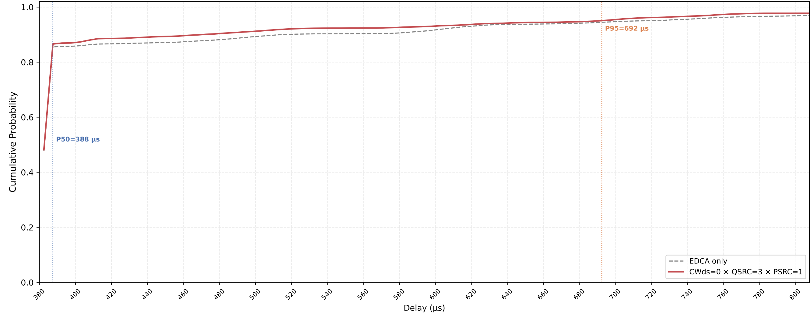
P-EDCA STA VO Delay CDF — CWds=0 × QSRC=3 × PSRC=1 nSta=30, nPedca=15, 0.1Mbps, avg of 10 runs
