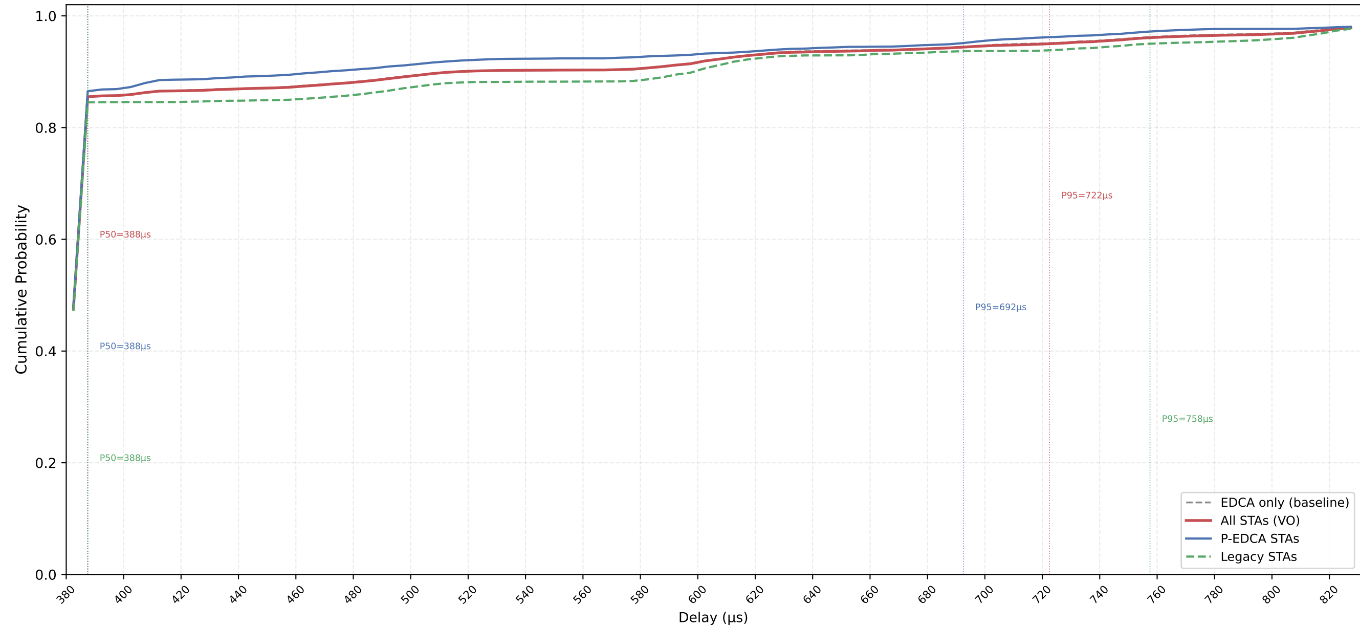
VO Delay CDF — P-EDCA / Legacy / All | CWds=0 × QSRC=3 × PSRC=2 nSta=30, nPedca=15/30, 0.1Mbps, avg of 10 runs
