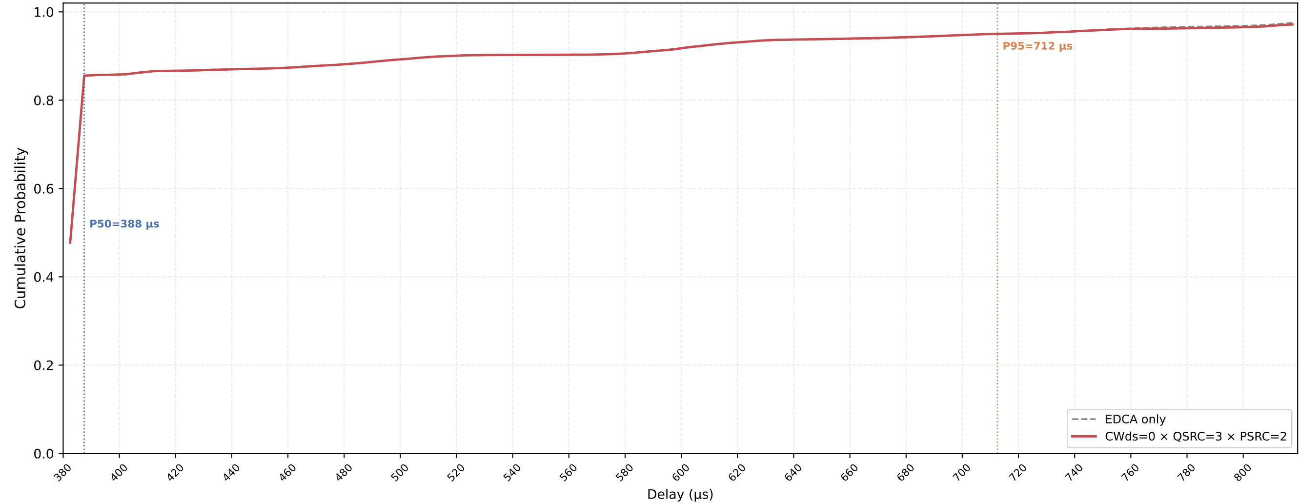
P-EDCA STA VO Delay CDF — CWds=0 × QSRC=3 × PSRC=2 nSta=30, nPedca=30, 0.1Mbps, avg of 10 runs
