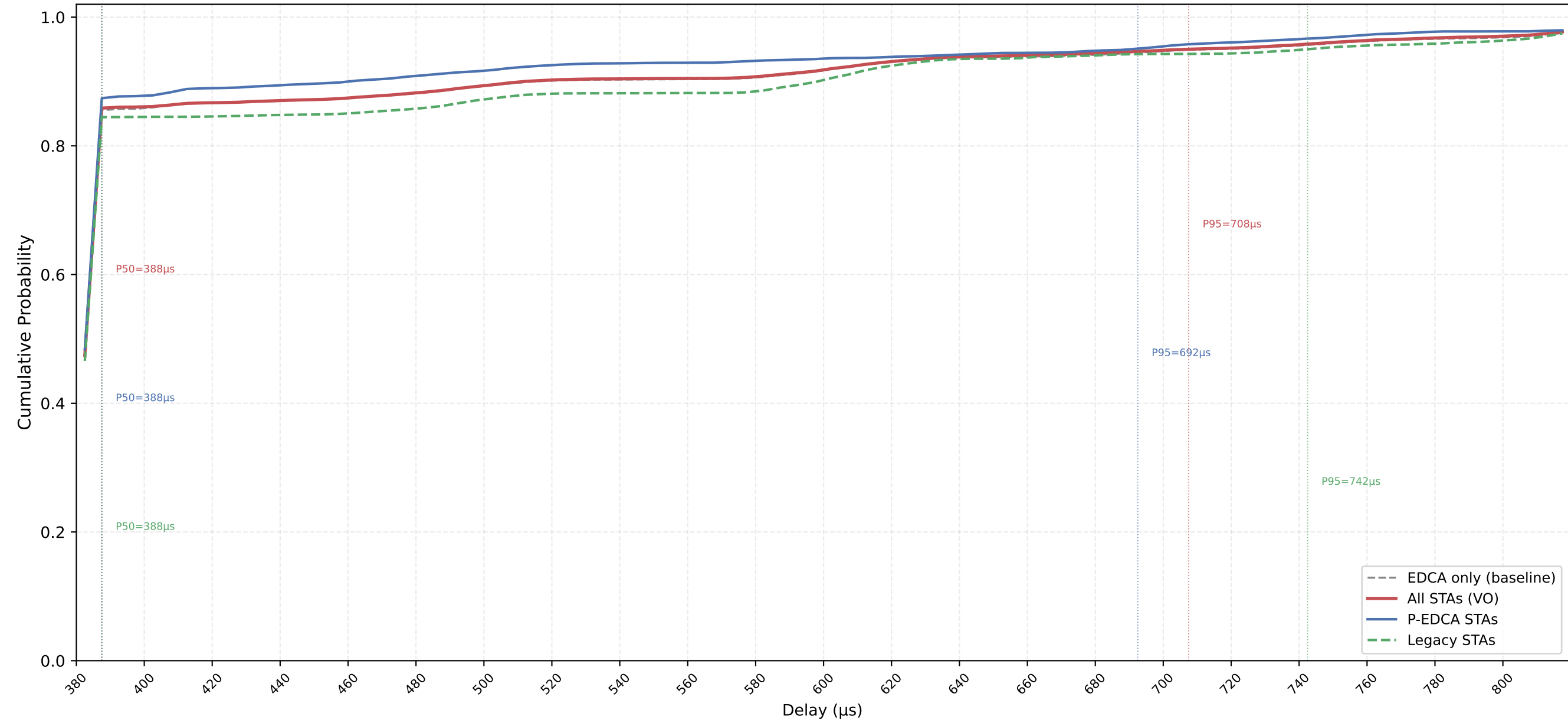
VO Delay CDF — P-EDCA / Legacy / All | CWds=0 × QSRC=3 × PSRC=3 nSta=30, nPedca=15/30, 0.1Mbps, avg of 10 runs
