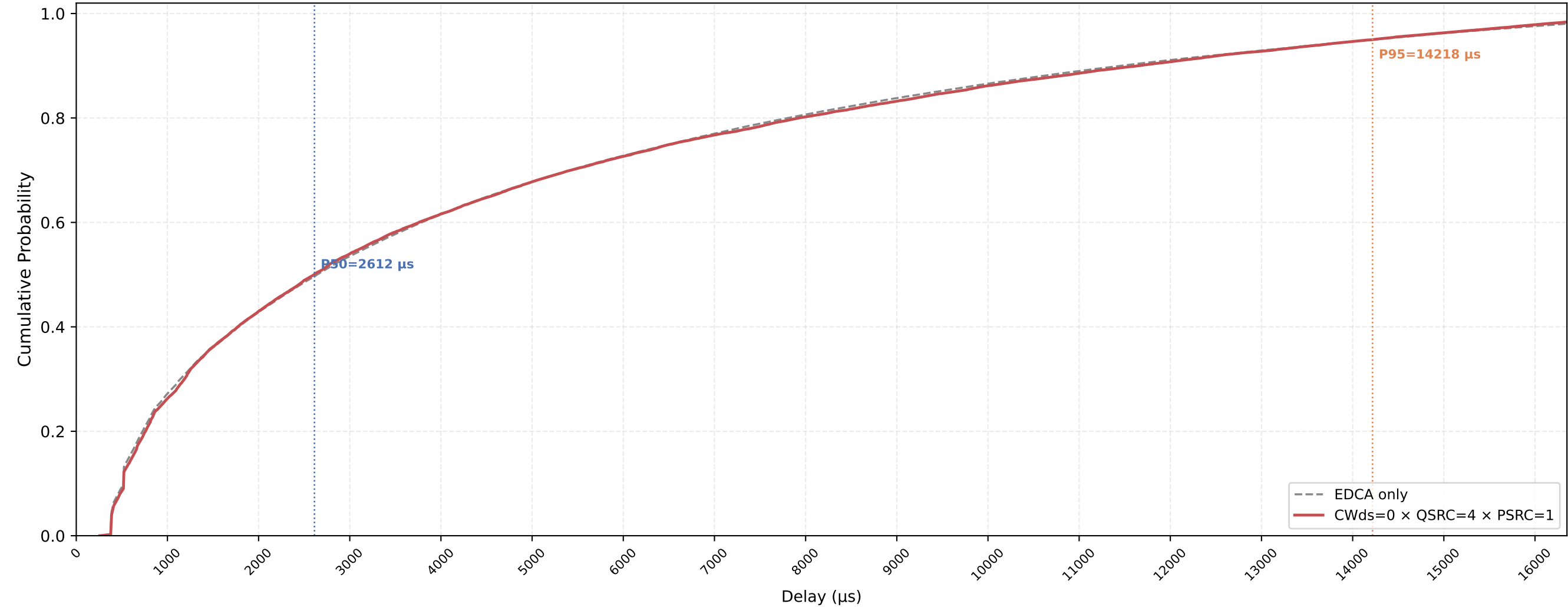
P-EDCA STA VO Delay CDF — CWds=0 × QSRC=4 × PSRC=1 nSta=30, nPedca=5, 0.5Mbps, avg of 10 runs
