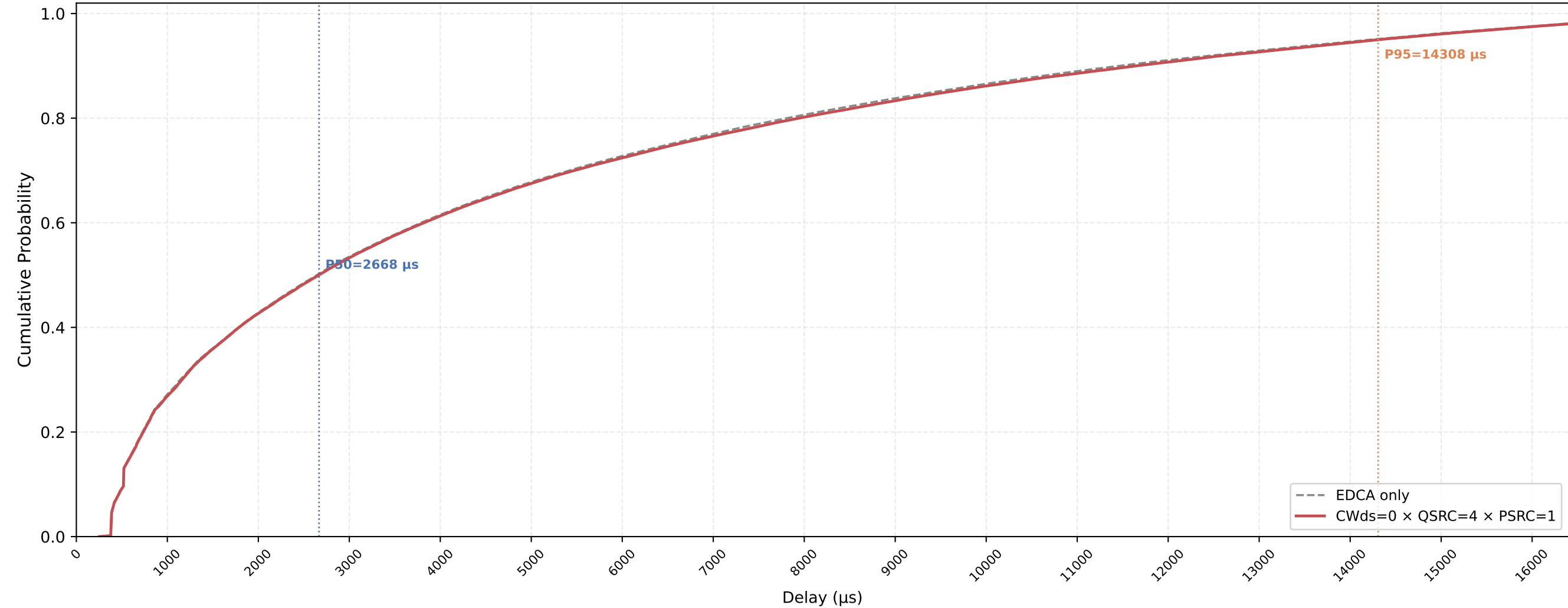
VO (all STAs) Delay CDF — CWds=0 × QSRC=4 × PSRC=1 nSta=30, nPedca=5, 0.5Mbps, avg of 10 runs
