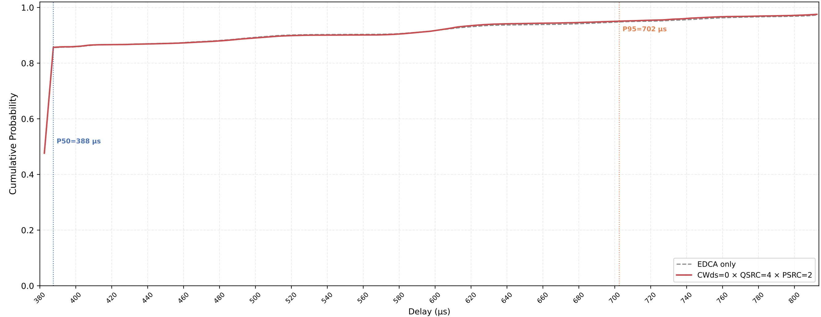
Legacy STA VO Delay CDF — CWds=0 × QSRC=4 × PSRC=2 nSta=30, nPedca=5, 0.1Mbps, avg of 10 runs
