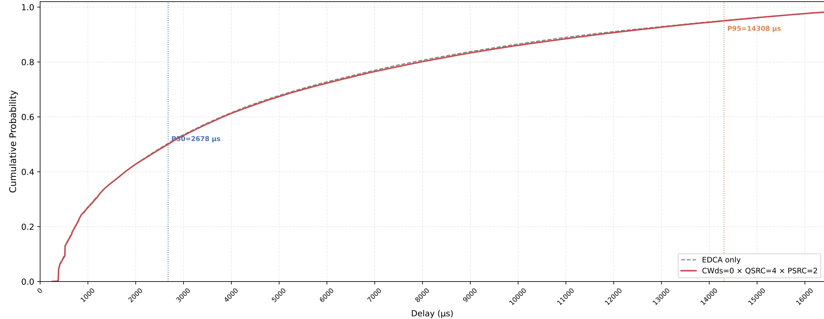
VO (all STAs) Delay CDF — CWds=0 × QSRC=4 × PSRC=2 nSta=30, nPedca=15, 0.5Mbps, avg of 10 runs
