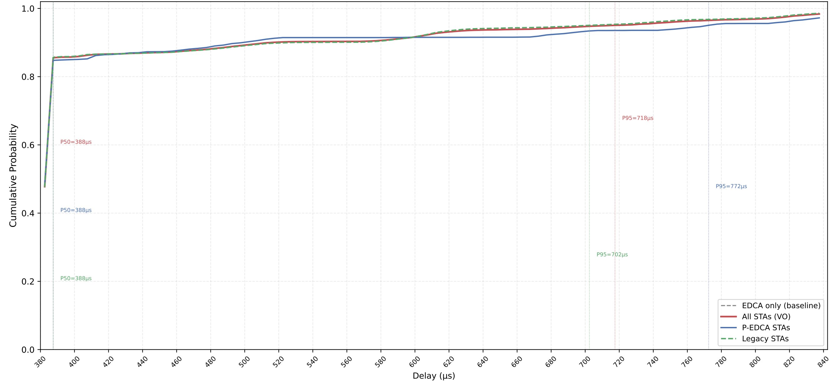
VO Delay CDF — P-EDCA / Legacy / All | CWds=0 × QSRC=4 × PSRC=3 nSta=30, nPedca=5/30, 0.1Mbps, avg of 10 runs
