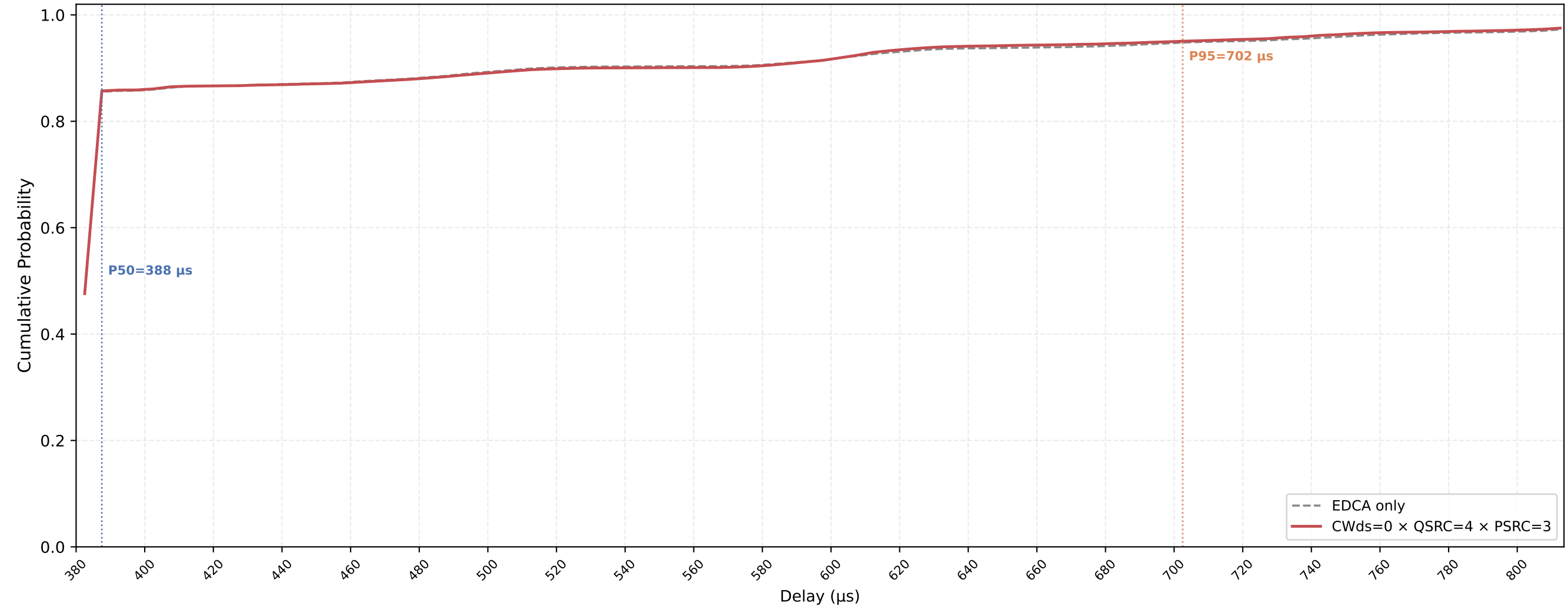
Legacy STA VO Delay CDF — CWds=0 × QSRC=4 × PSRC=3 nSta=30, nPedca=5, 0.1Mbps, avg of 10 runs
