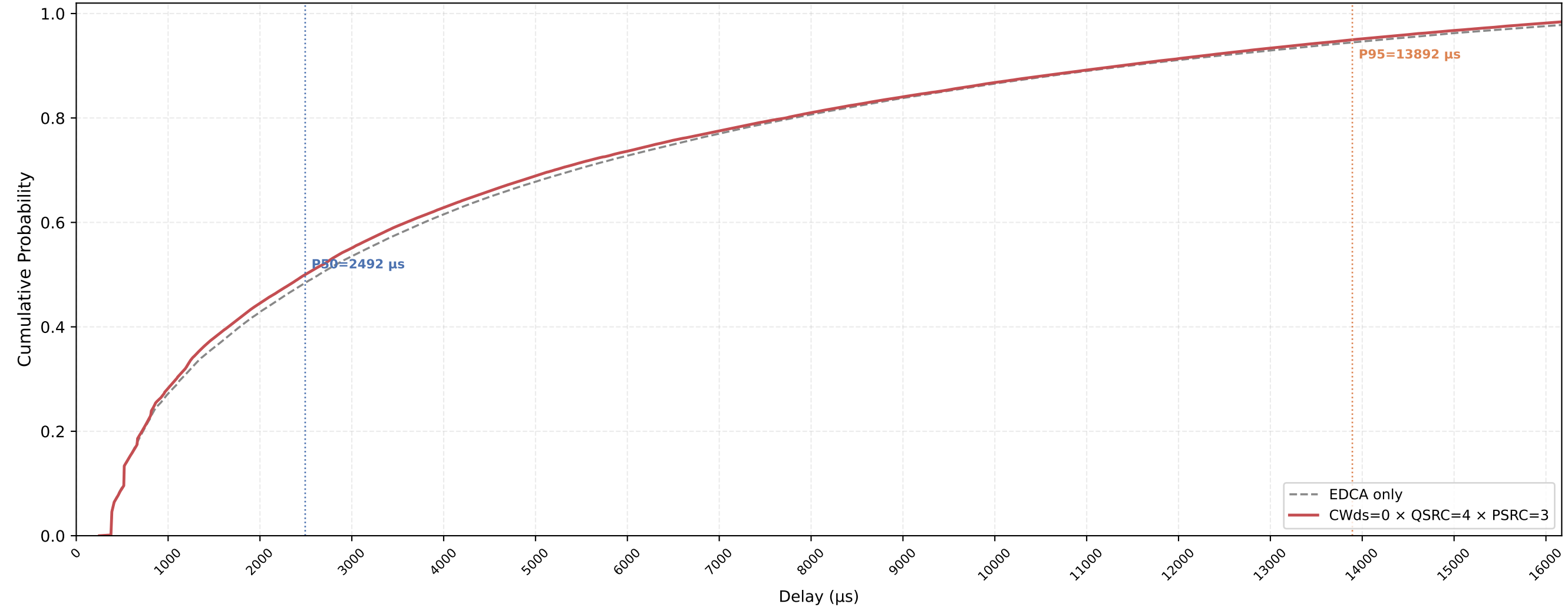
P-EDCA STA VO Delay CDF — CWds=0 × QSRC=4 × PSRC=3 nSta=30, nPedca=15, 0.5Mbps, avg of 10 runs
