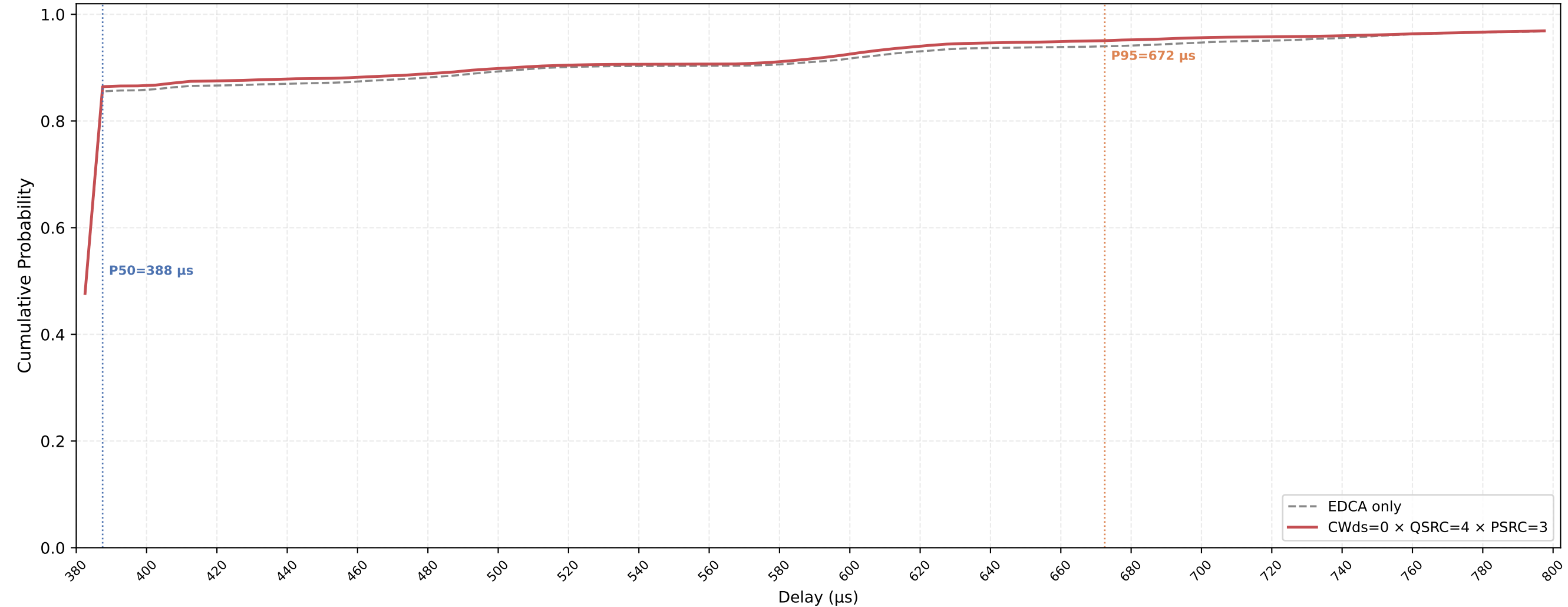
P-EDCA STA VO Delay CDF — CWds=0 × QSRC=4 × PSRC=3 nSta=30, nPedca=30, 0.1Mbps, avg of 10 runs
