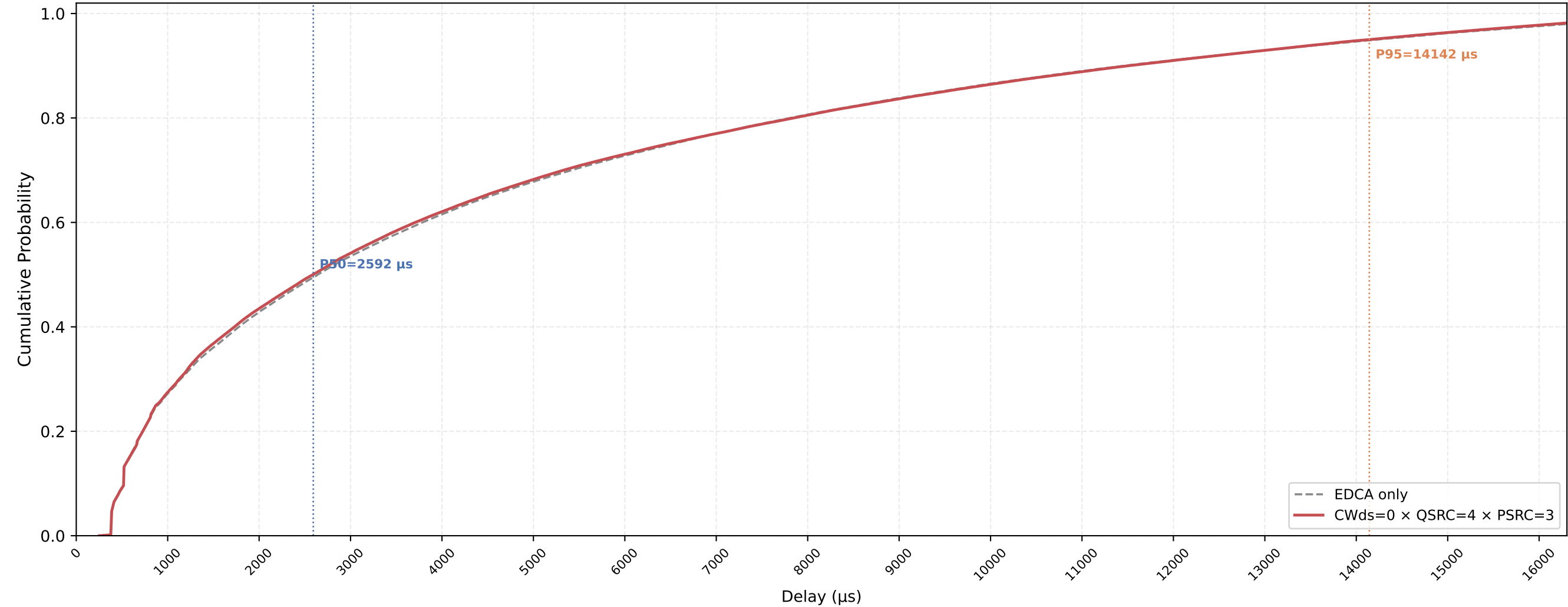
VO (all STAs) Delay CDF — CWds=0 × QSRC=4 × PSRC=3 nSta=30, nPedca=15, 0.5Mbps, avg of 10 runs
