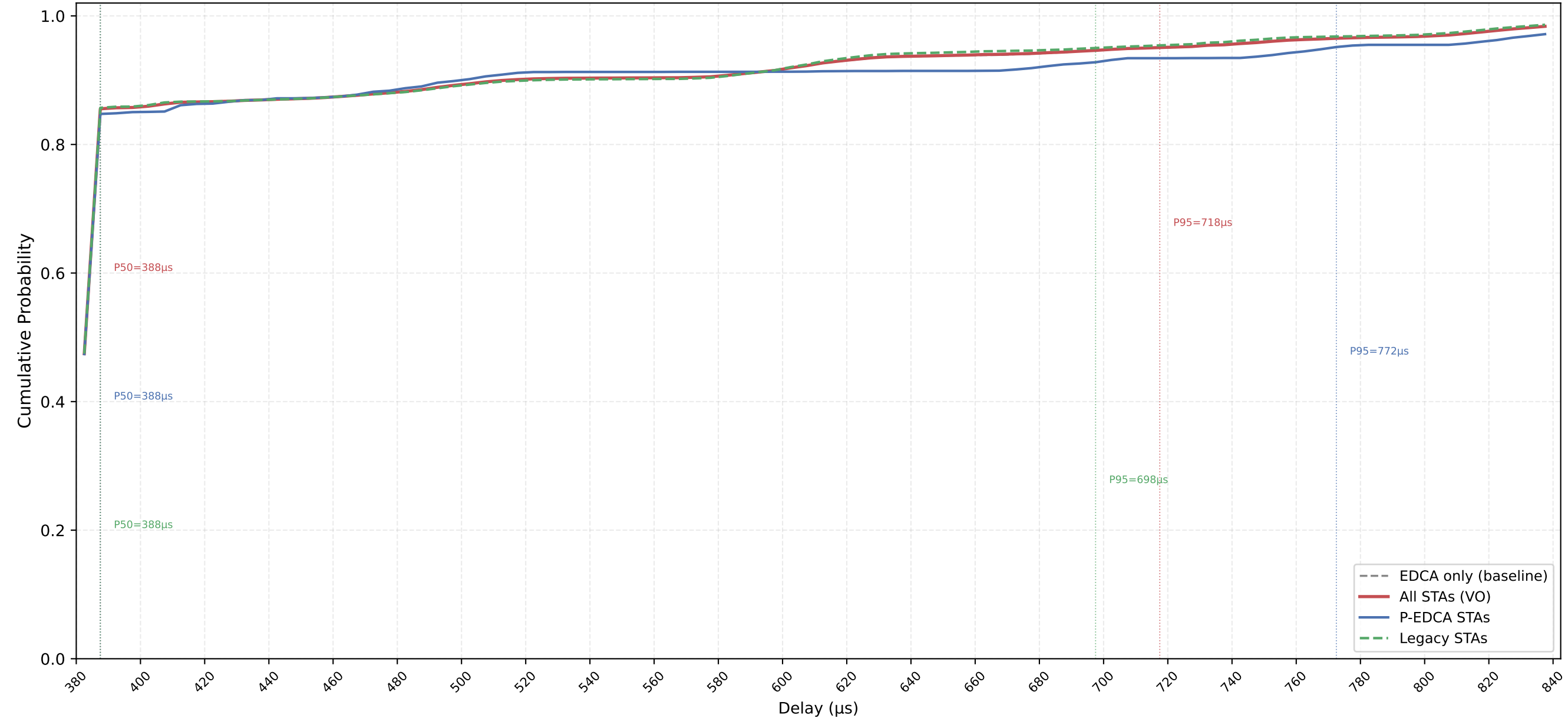
VO Delay CDF — P-EDCA / Legacy / All | CWds=0 × QSRC=5 × PSRC=1 nSta=30, nPedca=5/30, 0.1Mbps, avg of 10 runs
