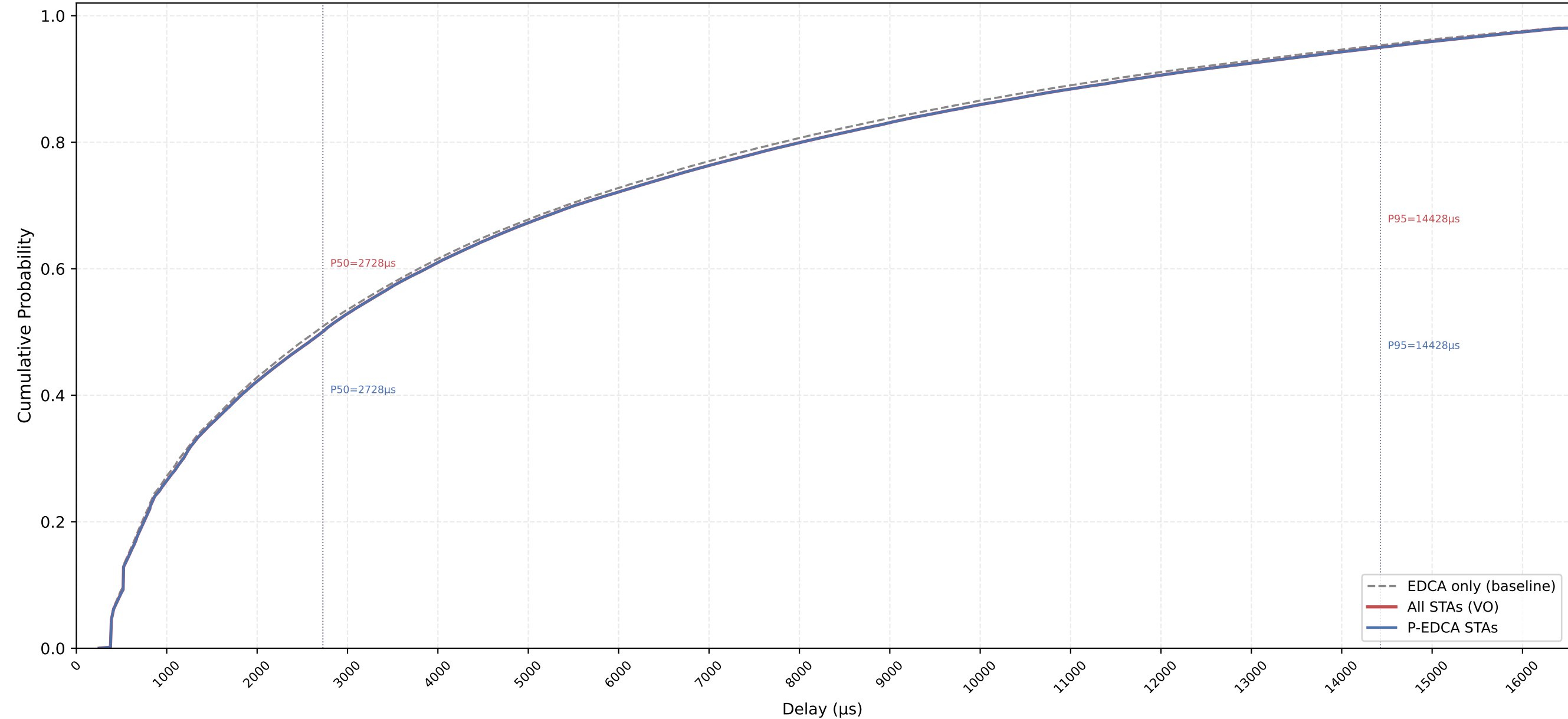
VO Delay CDF — P-EDCA / Legacy / All | CWds=0 × QSRC=5 × PSRC=1 nSta=30, nPedca=30/30, 0.5Mbps, avg of 10 runs
