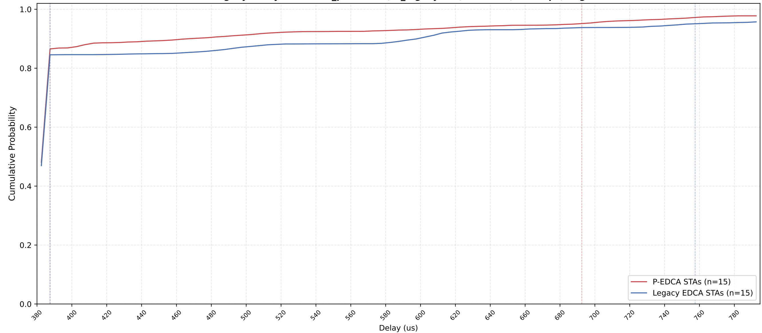
P-EDCA vs Legacy Delay CDF — n_pedca=15, n_legacy=15, nSta=30, 0.1Mbps, avg of 10 runs
