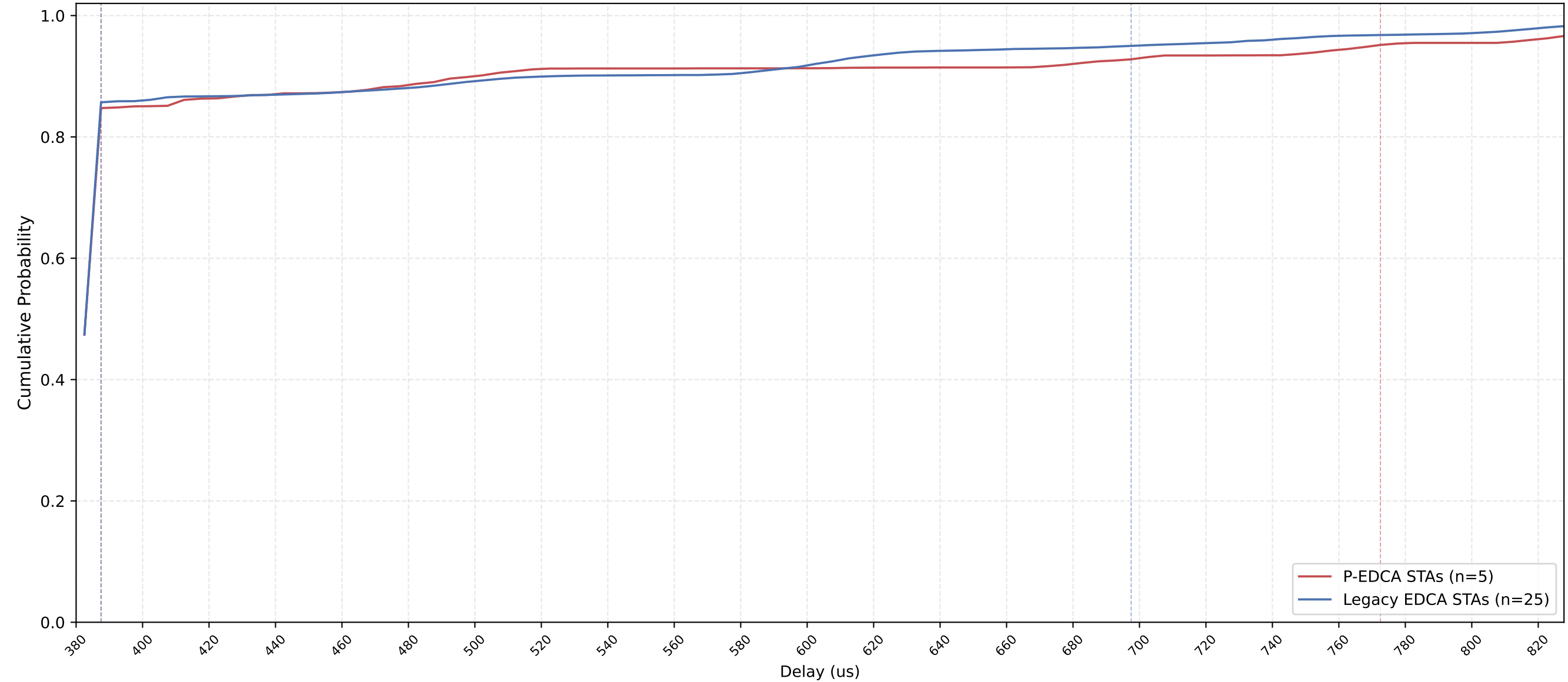
P-EDCA vs Legacy Delay CDF — n_pedca=5, n_legacy=25, nSta=30, 0.1Mbps, avg of 10 runs
