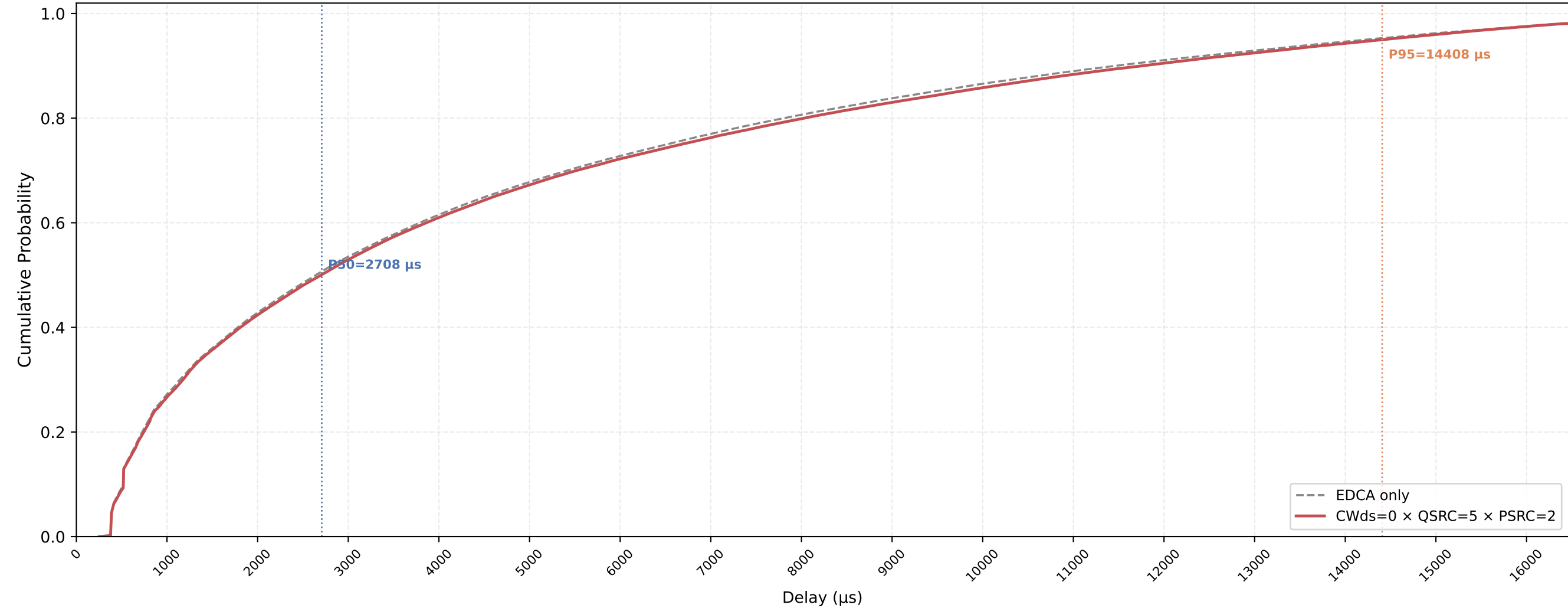
VO (all STAs) Delay CDF — CWds=0 × QSRC=5 × PSRC=2 nSta=30, nPedca=15, 0.5Mbps, avg of 10 runs
