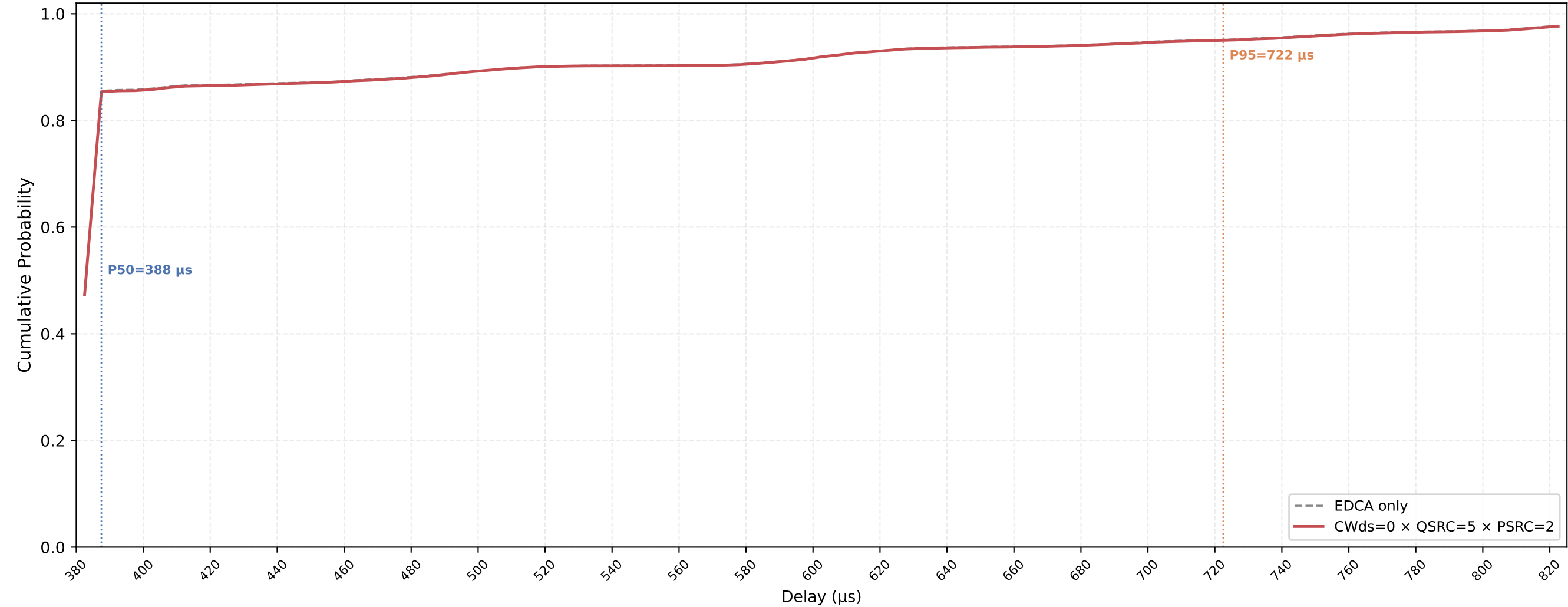
VO (all STAs) Delay CDF — CWds=0 × QSRC=5 × PSRC=2 nSta=30, nPedca=30, 0.1Mbps, avg of 10 runs
