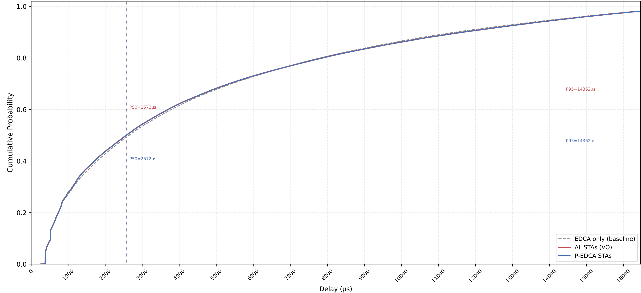
VO Delay CDF — P-EDCA / Legacy / All | CWds=0 × QSRC=5 × PSRC=3 nSta=30, nPedca=30/30, 0.5Mbps, avg of 10 runs
