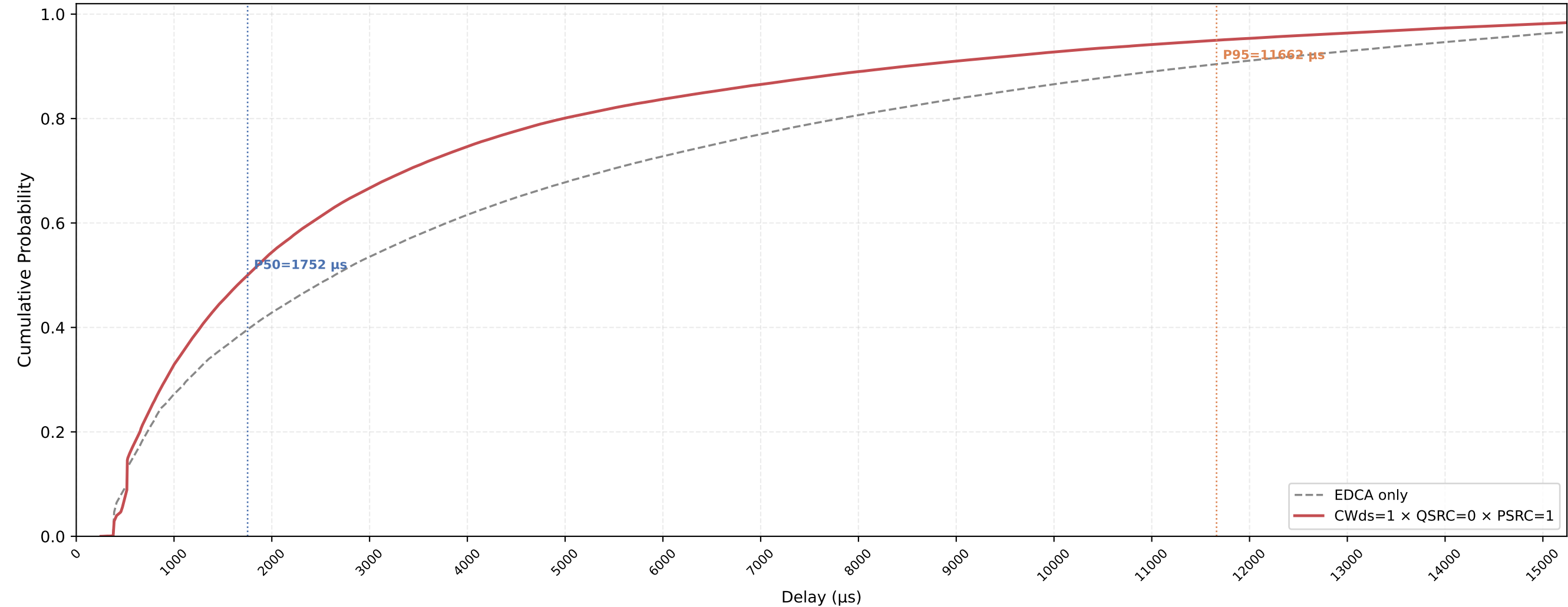
VO (all STAs) Delay CDF — CWds=1 × QSRC=0 × PSRC=1 nSta=30, nPedca=15, 0.5Mbps, avg of 10 runs
