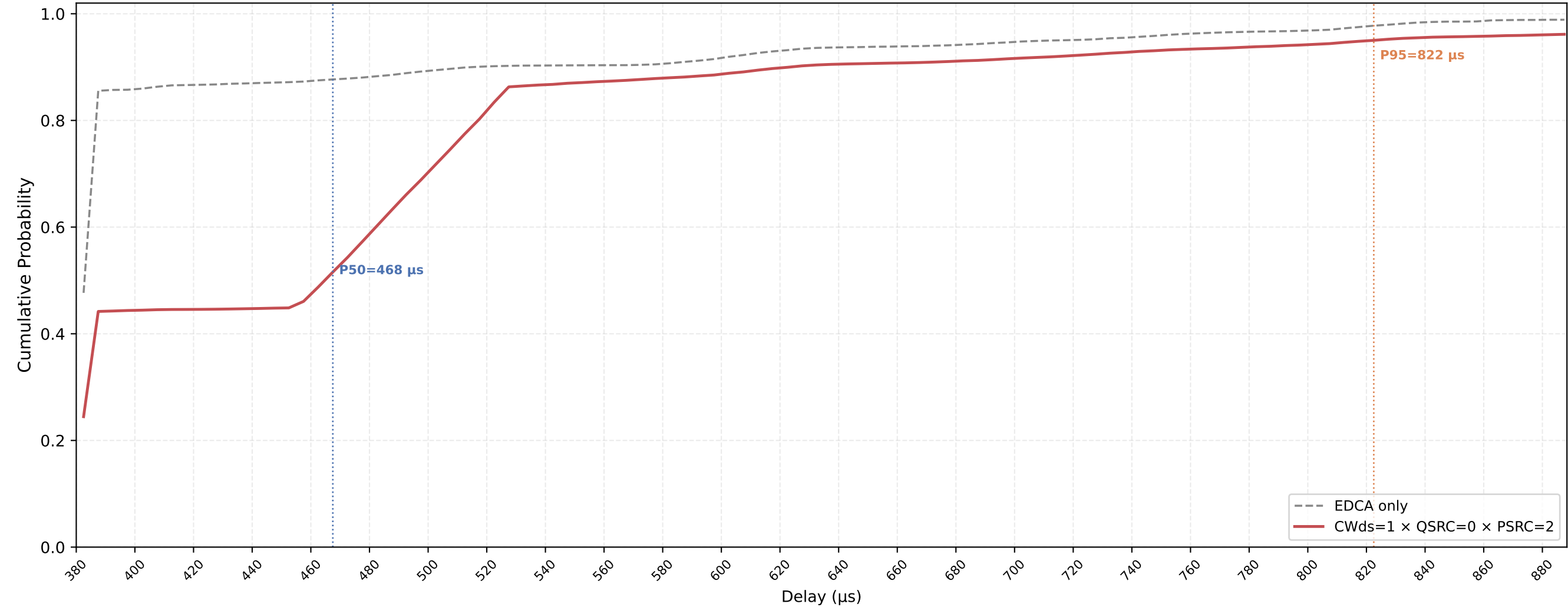
VO (all STAs) Delay CDF — CWds=1 × QSRC=0 × PSRC=2 nSta=30, nPedca=15, 0.1Mbps, avg of 10 runs
