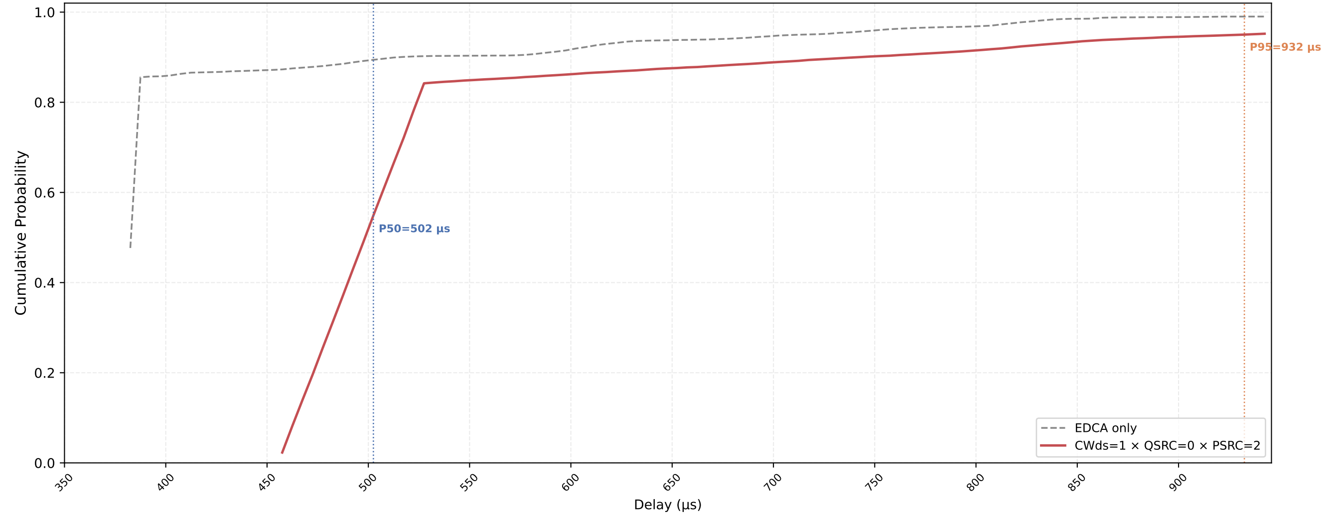
VO (all STAs) Delay CDF — CWds=1 × QSRC=0 × PSRC=2 nSta=30, nPedca=30, 0.1Mbps, avg of 10 runs
