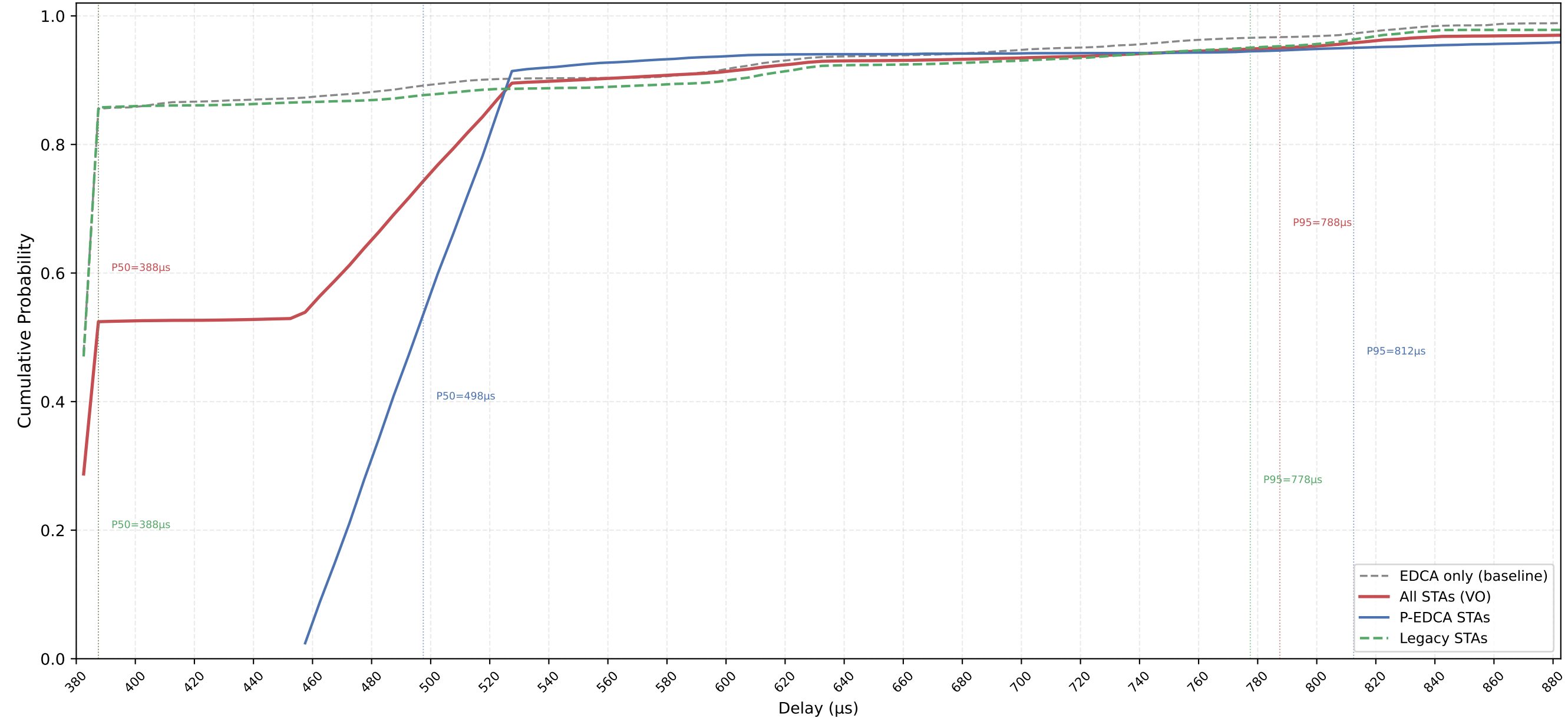
VO Delay CDF — P-EDCA / Legacy / All | CWds=1 × QSRC=0 × PSRC=3 nSta=30, nPedca=15/30, 0.1Mbps, avg of 10 runs
