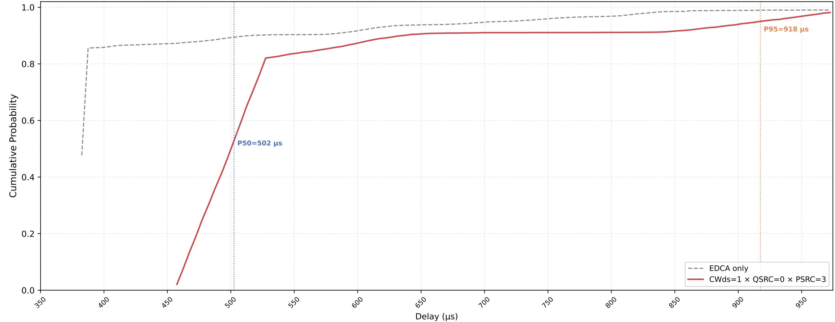
P-EDCA STA VO Delay CDF — CWds=1 × QSRC=0 × PSRC=3 nSta=30, nPedca=5, 0.1Mbps, avg of 10 runs
