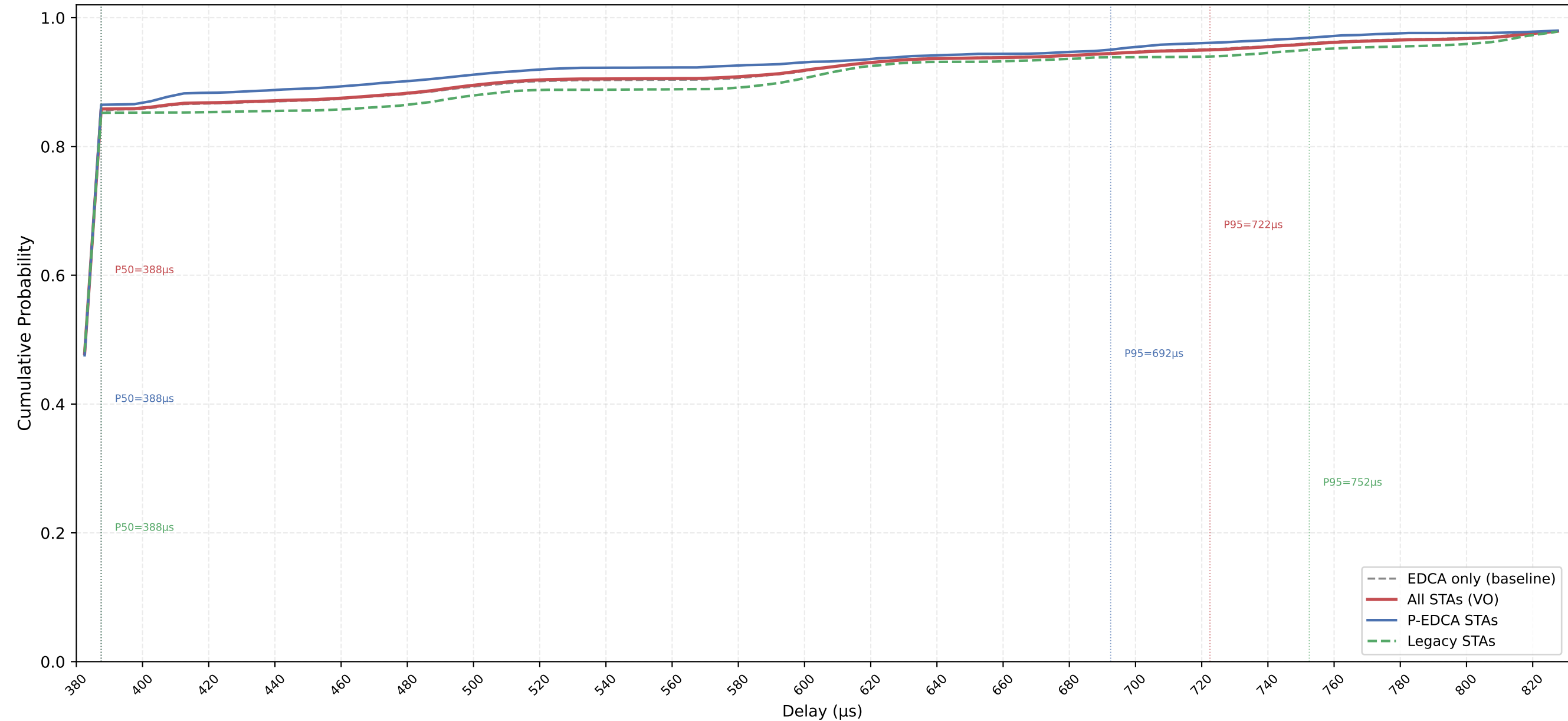
VO Delay CDF — P-EDCA / Legacy / All | CWds=1 × QSRC=1 × PSRC=1 nSta=30, nPedca=15/30, 0.1Mbps, avg of 10 runs
