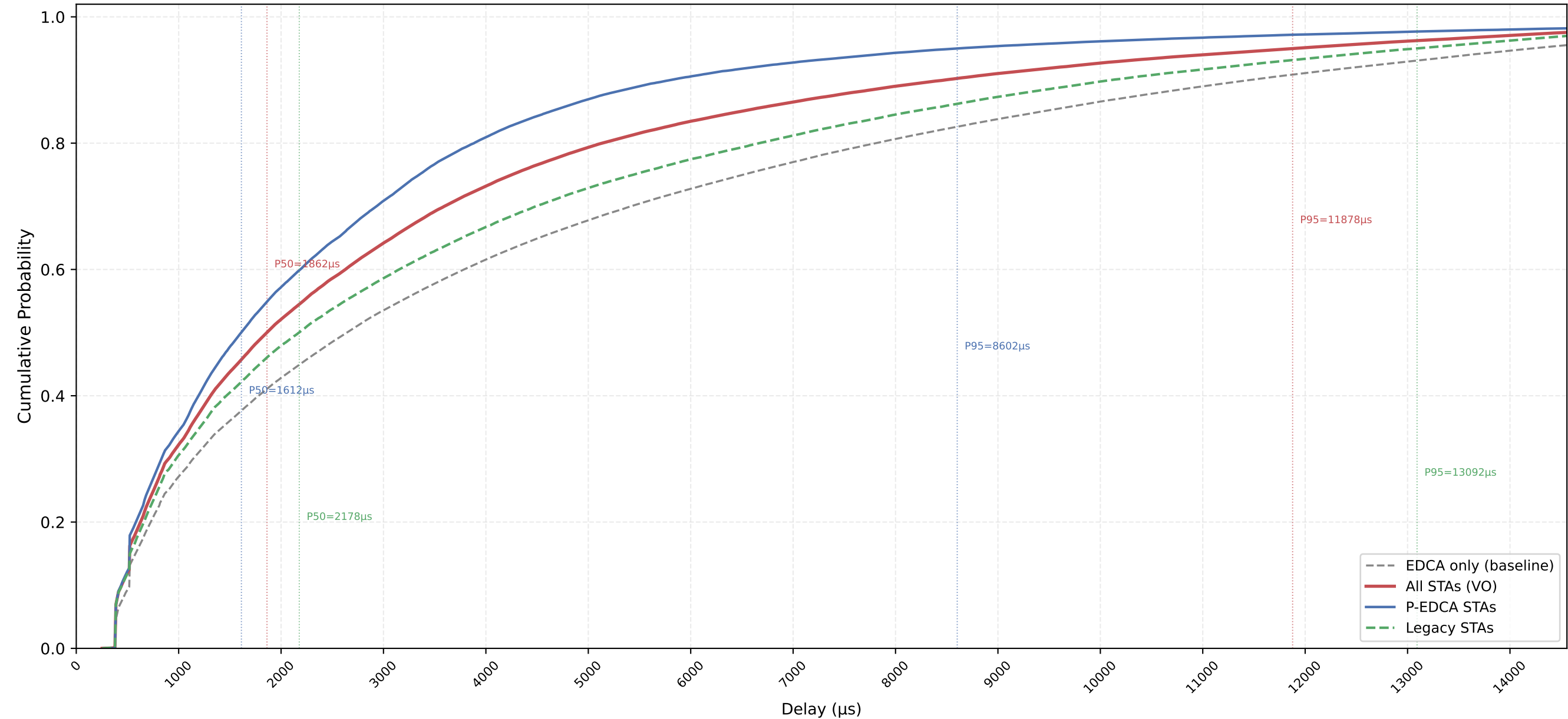
VO Delay CDF — P-EDCA / Legacy / All | CWds=1 × QSRC=1 × PSRC=1 nSta=30, nPedca=15/30, 0.5Mbps, avg of 10 runs
