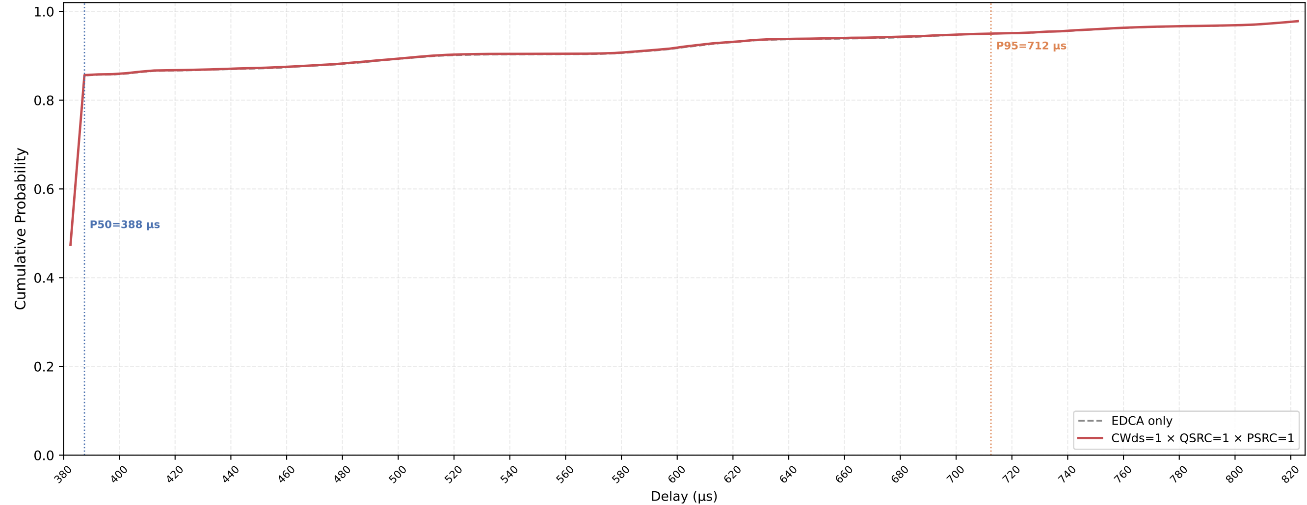
VO (all STAs) Delay CDF — CWds=1 × QSRC=1 × PSRC=1 nSta=30, nPedca=5, 0.1Mbps, avg of 10 runs
