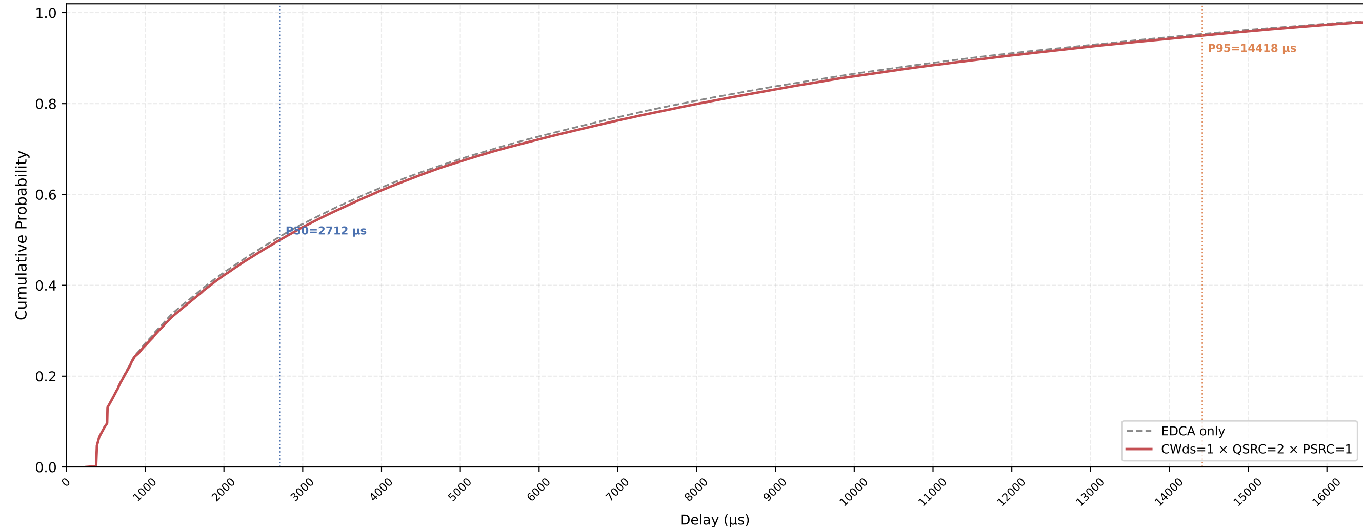
Legacy STA VO Delay CDF — CWds=1 × QSRC=2 × PSRC=1 nSta=30, nPedca=5, 0.5Mbps, avg of 10 runs
