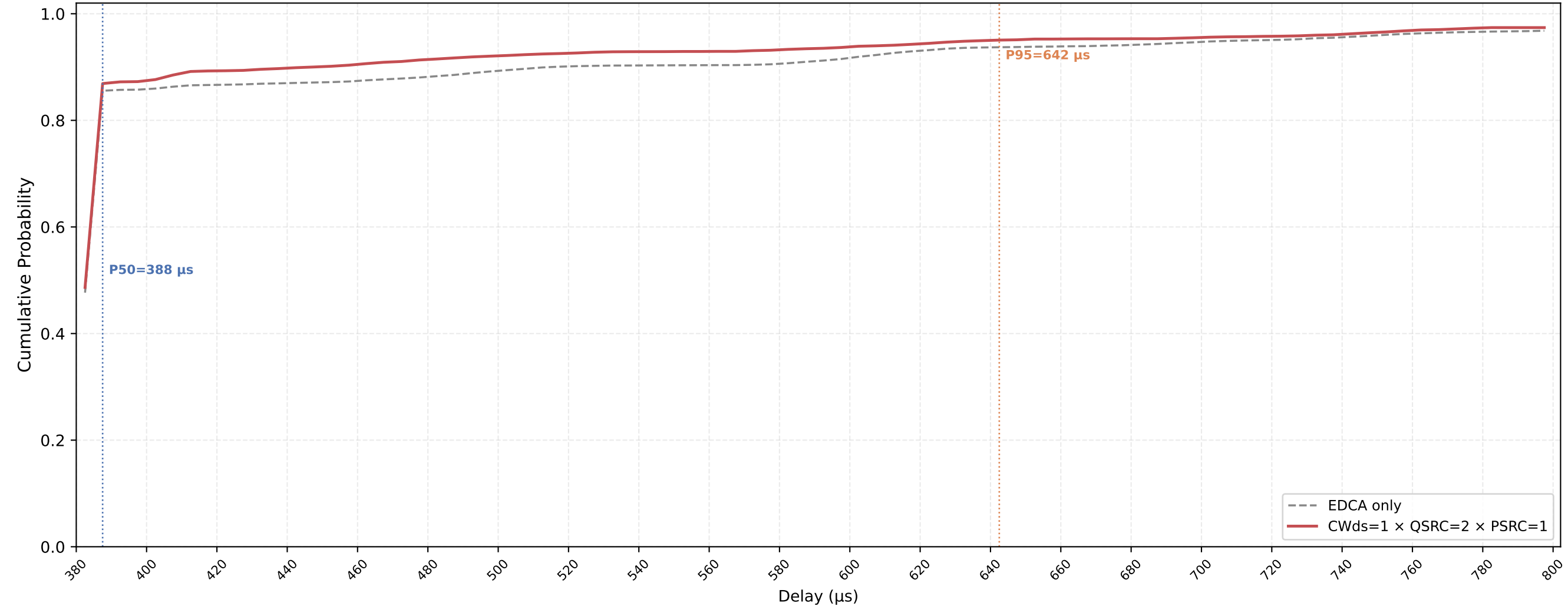
P-EDCA STA VO Delay CDF — CWds=1 × QSRC=2 × PSRC=1 nSta=30, nPedca=15, 0.1Mbps, avg of 10 runs
