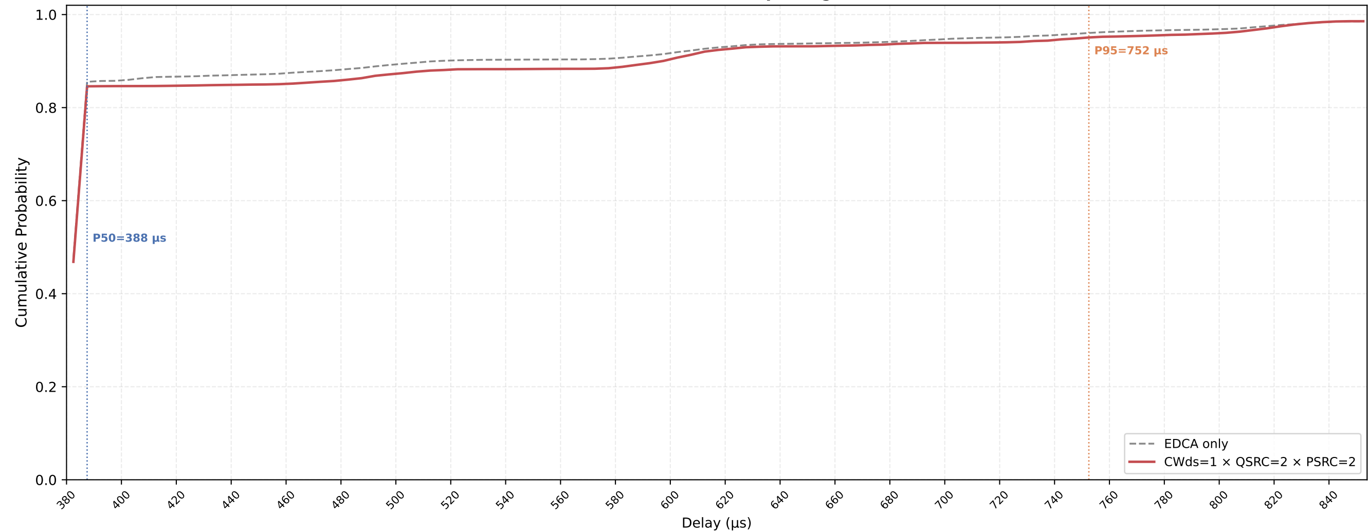
Legacy STA VO Delay CDF — CWds=1 × QSRC=2 × PSRC=2 nSta=30, nPedca=15, 0.1Mbps, avg of 10 runs
