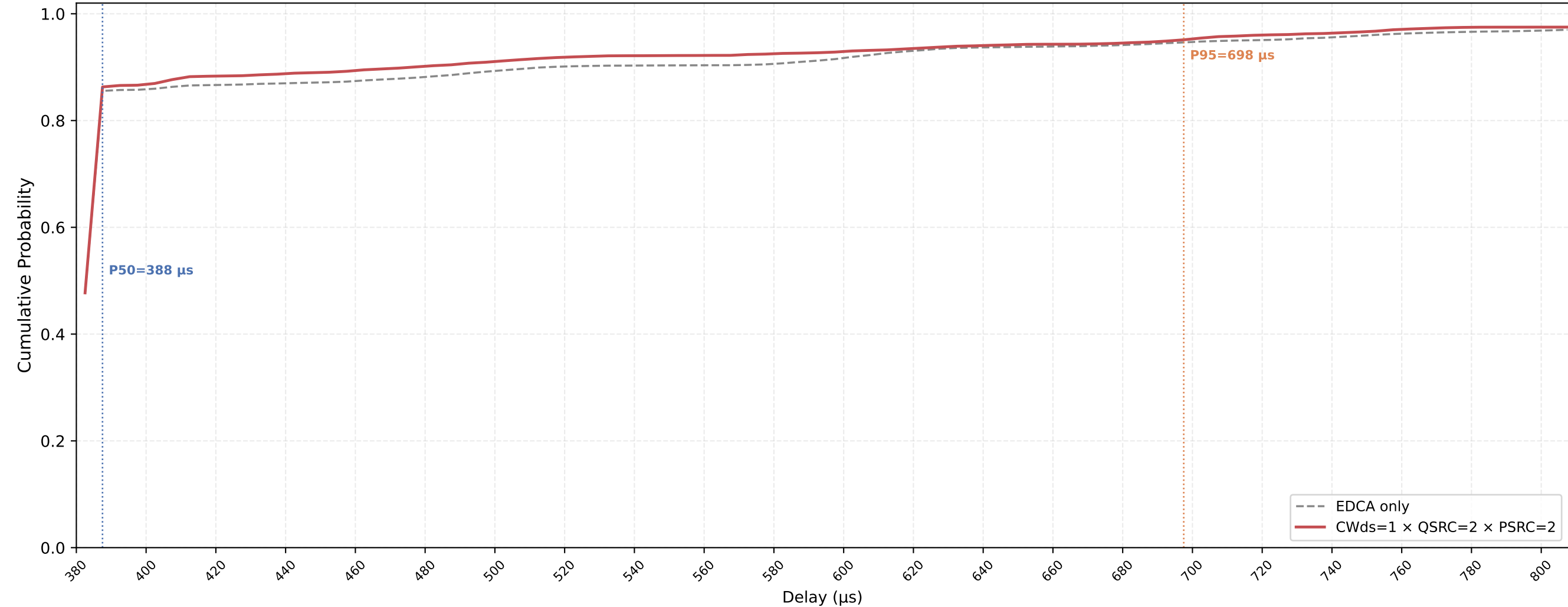
P-EDCA STA VO Delay CDF — CWds=1 × QSRC=2 × PSRC=2 nSta=30, nPedca=15, 0.1Mbps, avg of 10 runs
