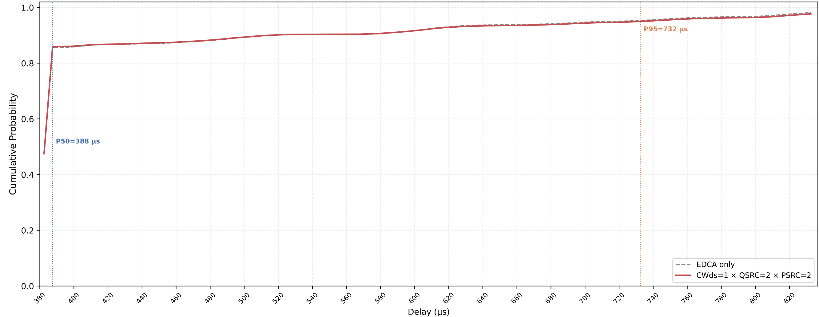
P-EDCA STA VO Delay CDF — CWds=1 × QSRC=2 × PSRC=2 nSta=30, nPedca=30, 0.1Mbps, avg of 10 runs
